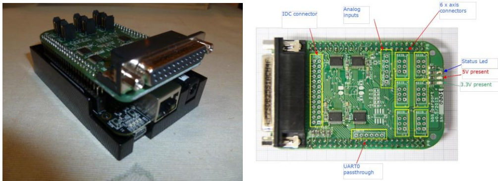
Figure 6. BeagleBone Black with bbb_parport
