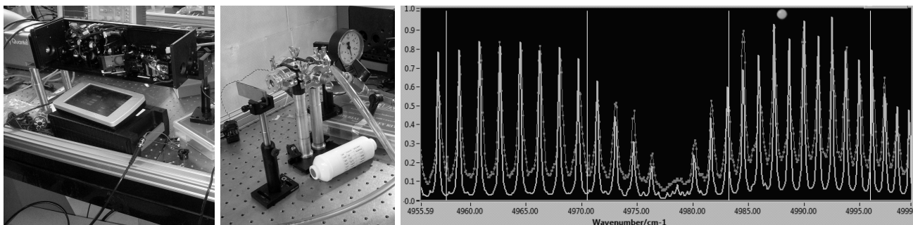
Figure 4. Left) The OPO opened during the test of the laser source of VULLI. Center) Photo-acoustic cell. Right) Theoretical (line) and experimental (circles and line) \text{CO}_2 absorption spectrum.
