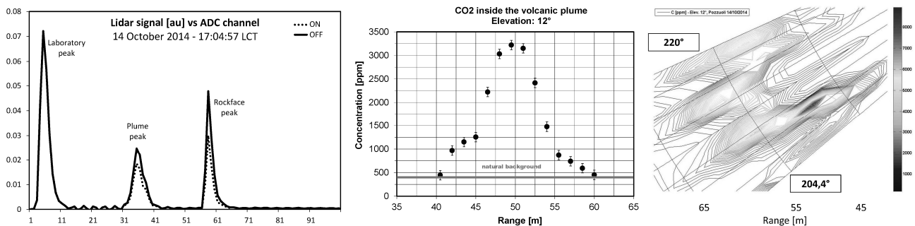
Figure 2. Example of: Left) lidar signal. Center) \text{CO}_2 profile. Right) Plume scan (the vent correspond to the grey spot).
