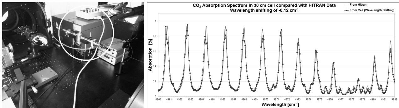
Figure 3. Left) Photo-acoustic cell (inside the white circle). Right) Theoretical (line) and experimental (circles and line) \text{CO}_2 absorption spectrum.
