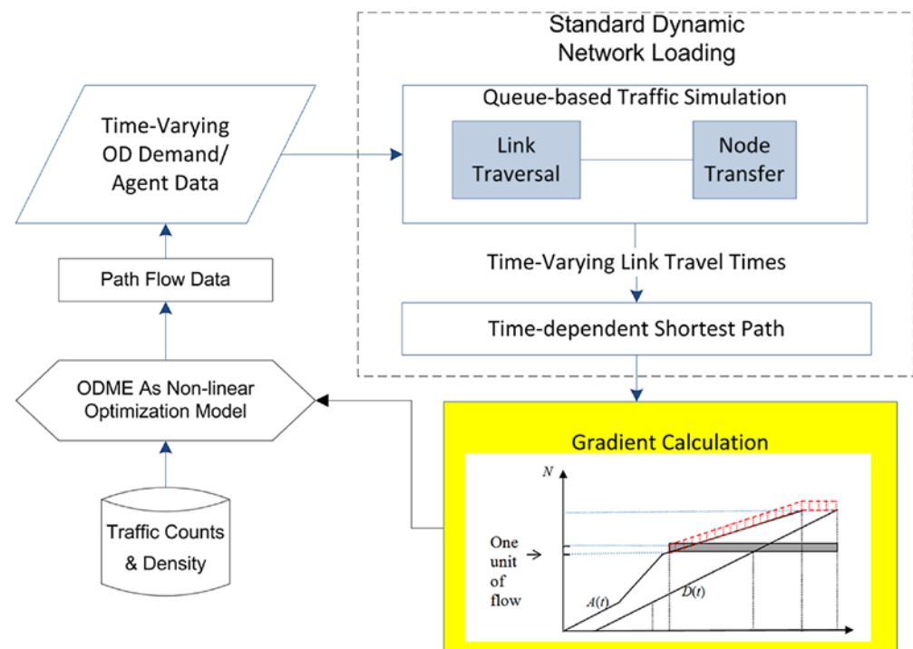
Figure 12. Single-level Origin-Destination Matrix Estimation (ODME) flowchart.
