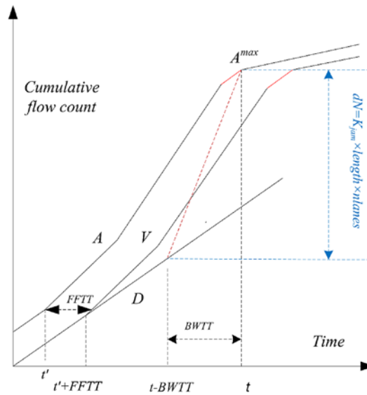
Figure 7. Illustration of cumulative arrival and departure curves A(t) and D(t) , and the shifted arrival curve V(t) .
