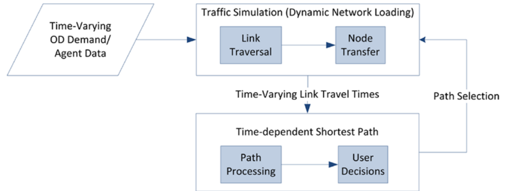
Figure 2. General simulation-based DTA modeling framework.
