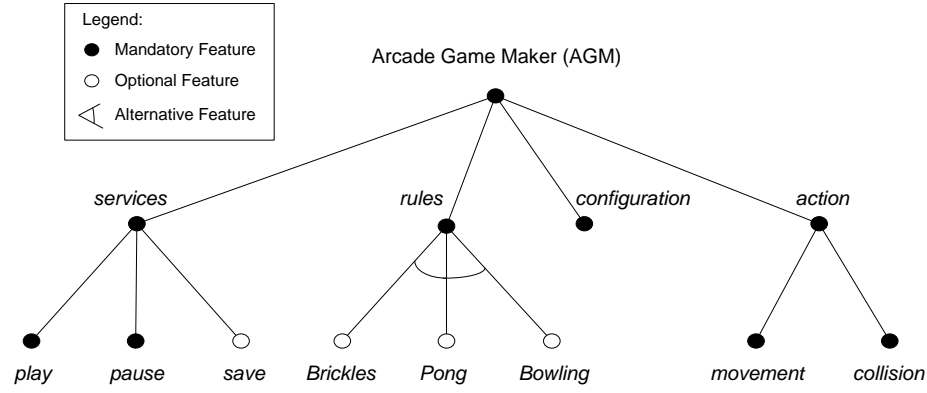
Figure 3: The Arcade Game Maker Feature Model.
