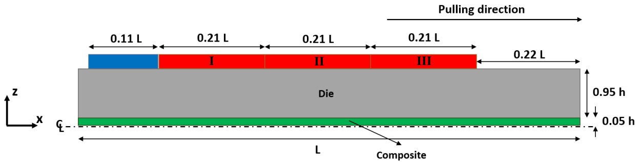
Figure 5: Normalized 2D schematic representation of half of the pultrusion domain (not to scale).
