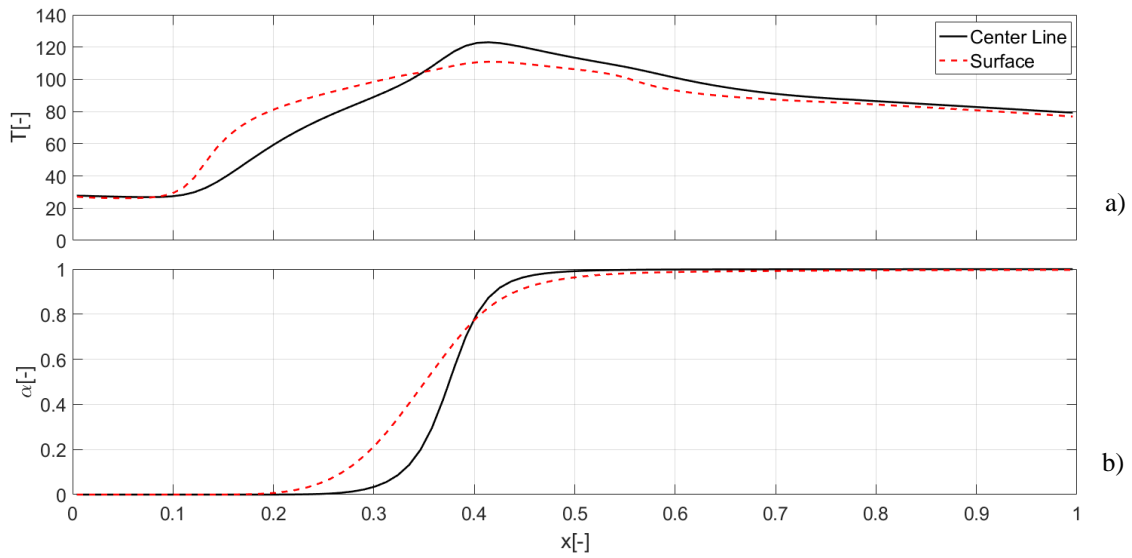
Figure 7: Comparison of normalized centerline and surface predictions: a) temperature, b) degree of cure.
