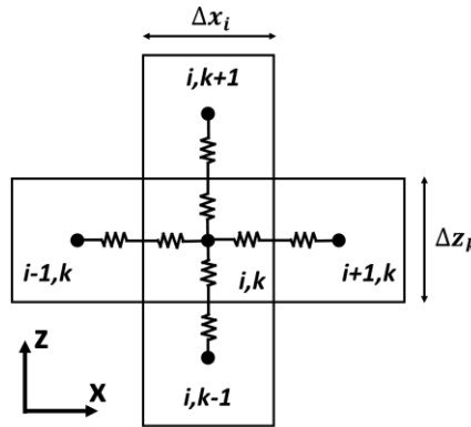
Figure 2: Schematic representation of indexing in the 2D domain (length-thickness plane) including thermal resistances (zigzag lines).
