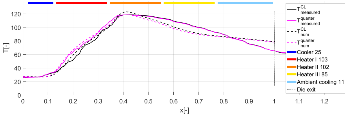
Figure 9: Comparison of measured and numerically predicted temperature profiles including the positions of cooler, heaters and ambient cooling along the longitudinal direction (normalized).
