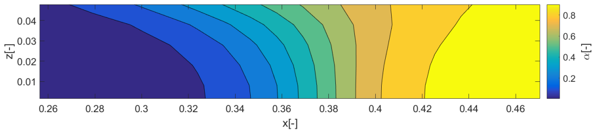
Figure 8: Normalized contour illustrating the evolution of the degree of cure (not to scale).
