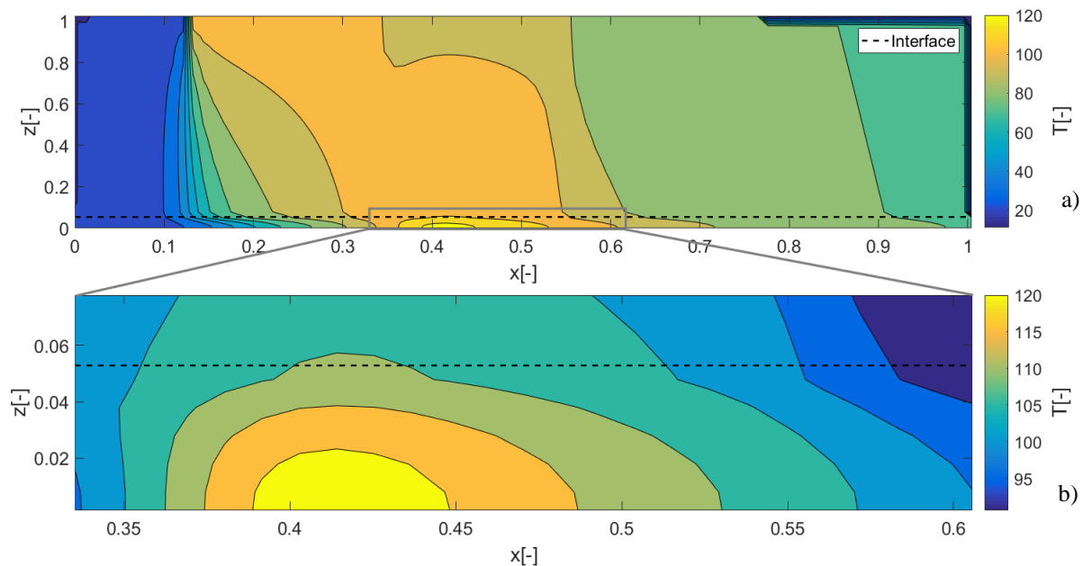
Figure 6: Normalized steady state temperature contour (not to scale): a) The whole 2D domain, b) Zoom, illustrating the exothermic heat generation inside the composite.
