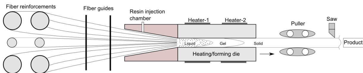
Figure 1: Schematic representation of the Resin Injection Pultrusion (RIP) process.
