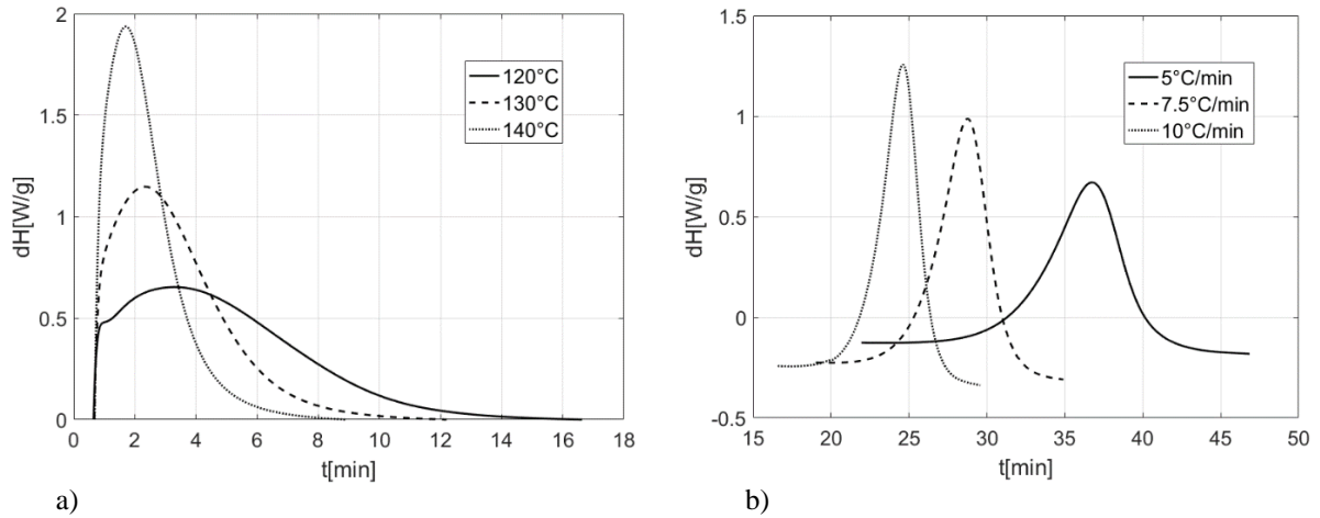
Figure 3: Heat flow curves from DSC experiments. a) Isothermal, b) dynamic.
