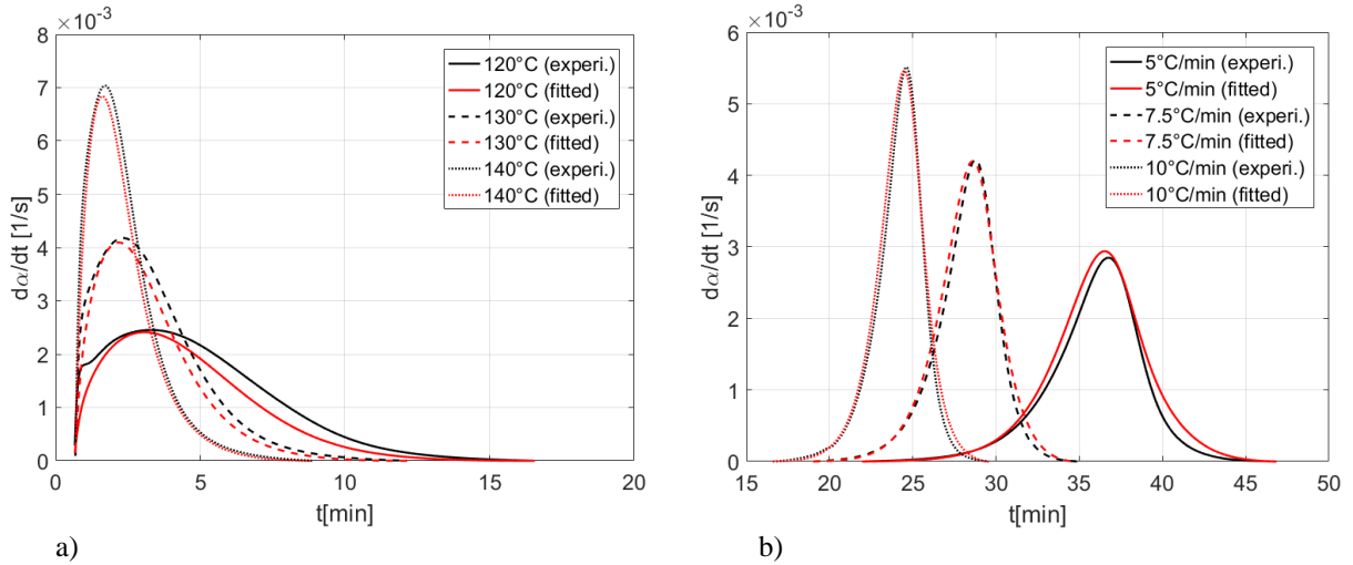
Figure 4: Comparison of experimental cure rate with CKM predictions (cf. Eq. (5) and Table 1). a) isothermal, b) dynamic.
