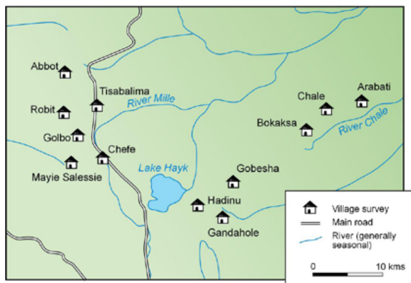
Figure 7 – Location of villages surveyed in South Wollo
