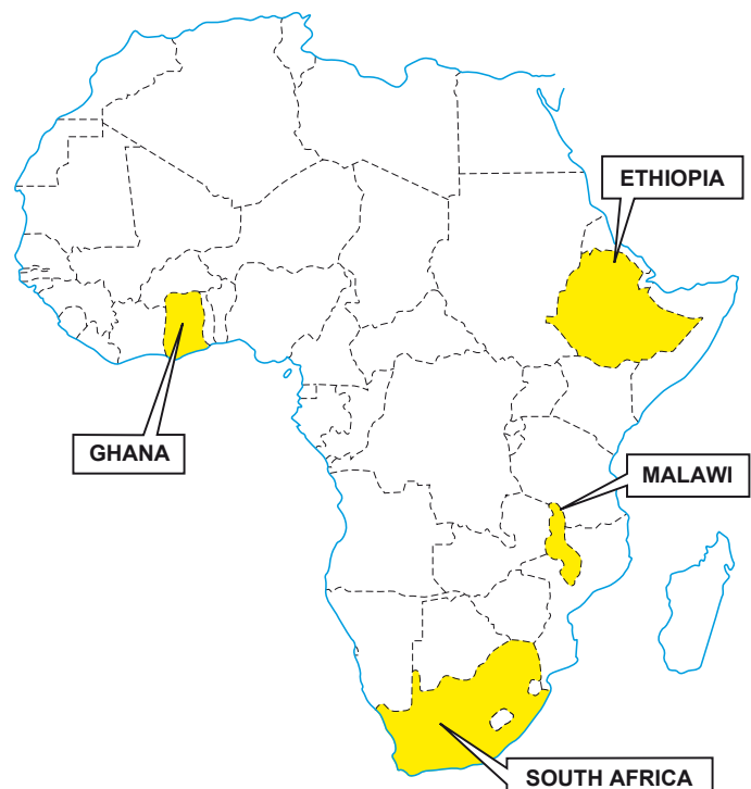
Figure 1 - Location of countries studied as part of this research
