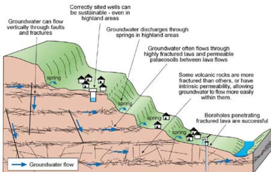
Figure 9 – Cross-section of groundwater flow in highland volcanic areas
