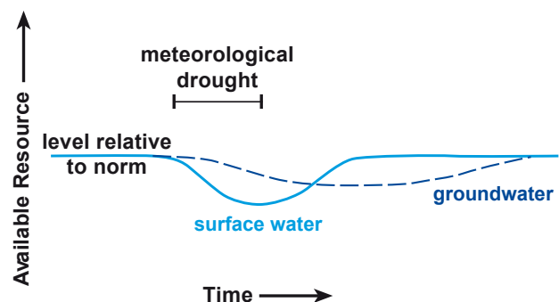
Figure 2 - The response of groundwater and surface water to meteorological drought. Groundwater resources respond slowly to changes in rainfall.
