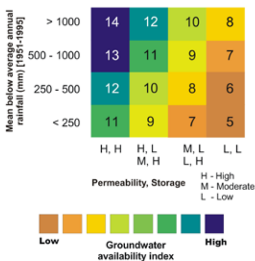
Figure 5 – Matrix used to evaluate groundwater availability during drought
