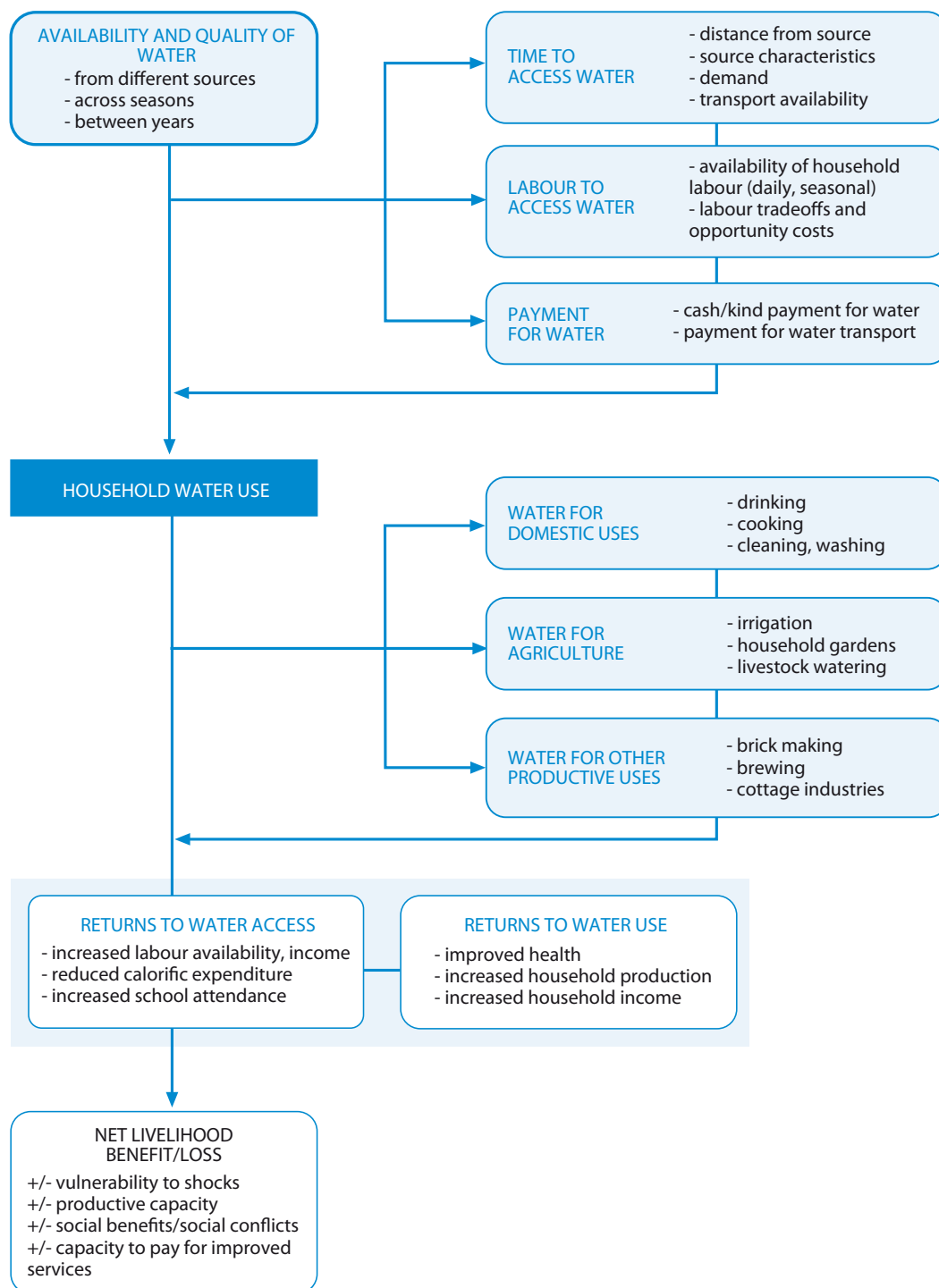
Figure 11 – Schematic diagram of the household water economy. Source: ODI 2002.
