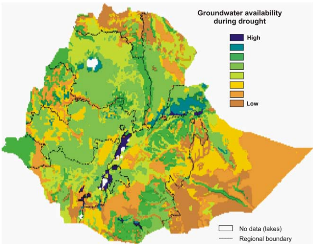
Figure 8 – Summary map - groundwater availability during drought
