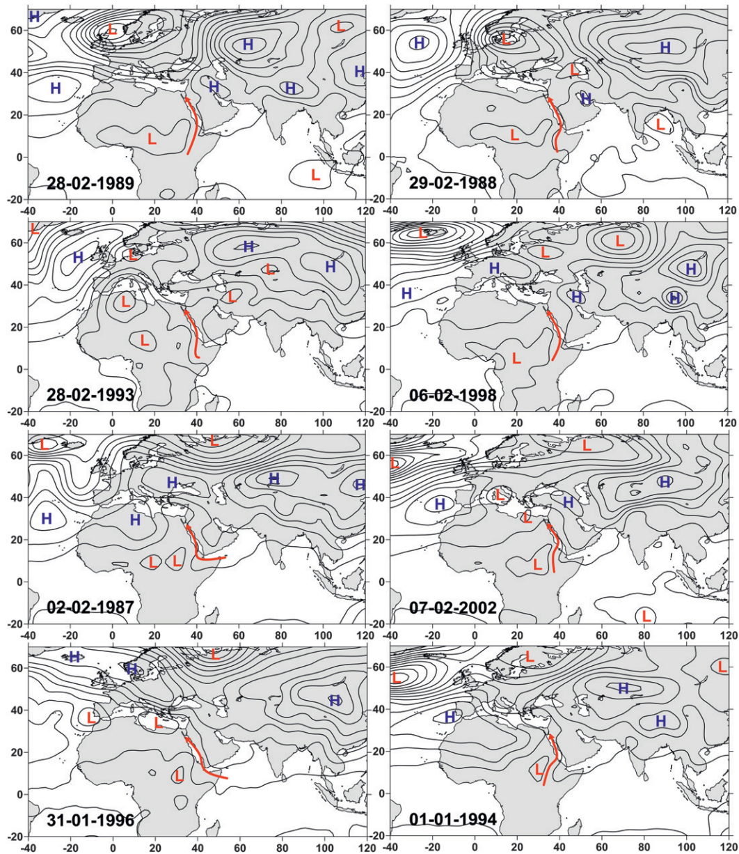
FIG. 10. Synoptic SLP maps (with the corresponding dates) during the eight highest daily winter LH + SH values. Manually drawn thick red lines show schematically the potential air mass routes toward the northern part of the Red Sea.
