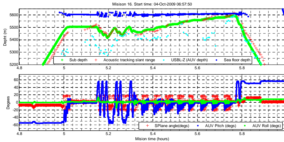
Figure 7. Mission 16, data from the deepest segment of the mission. Returns (red crosses in top plot) show similar characteristics to the mission in cruise JC027 - 6
