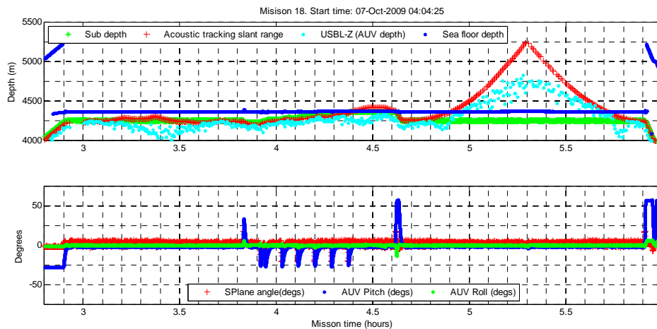
Figure 8. Mission 18 took place in conditions similar to those experienced in the JC027 missions. It can be seen that in this case the Linkquest telemetry worked reliably.
