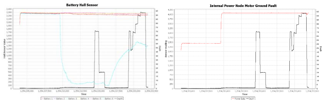
Figure 1 Battery Hall effect sensor readings (left) and Internal Power Node Motor Ground Fault (right) during Mission 14. The motor ground fault reads high and the Hall sensor low as soon as Autosub enters the water. Livingstone correctly detected the faults and localised them as soon as they occur.
