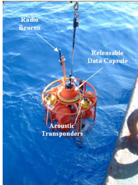
b – MYRTLE Deployment
