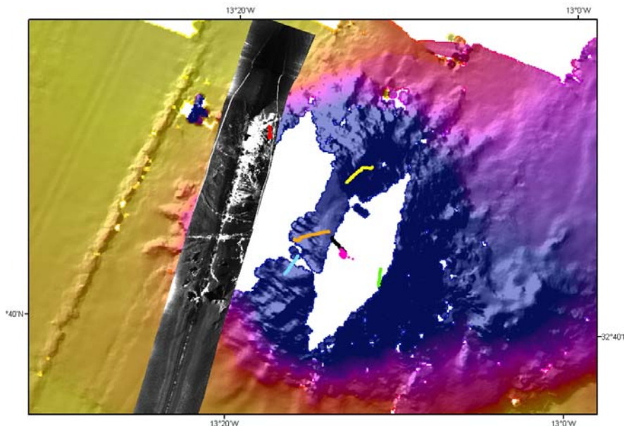
Map showing all dive sites during HyBIS trials on cruise D343. Background data are multibeam bathymetry and TOBI sidescan sonar imagery.
