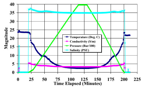
d – Internally Recorded Seabird Microcat CTD Data at 60 second intervals
