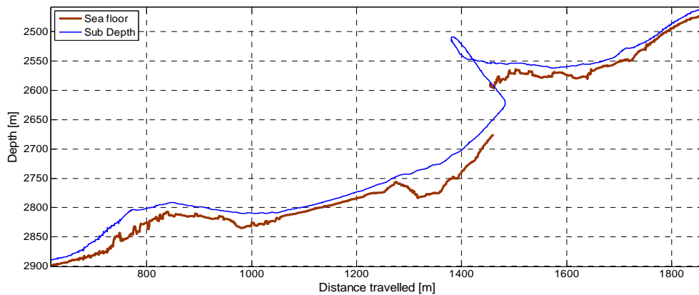
Figure 3. Ocean floor and Autosub6000 depth profile during part of the 10m altitude terrain following ascent of the Casablanca Seamount. Note collision avoidance behaviour after 1.4Km.
