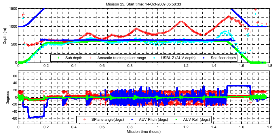
Figure 10. Mission 25, low 3m altitude survey on Casablanca Seamount top, at a depth of approximately 600m. The Tracking and telemetry worked reliably.
