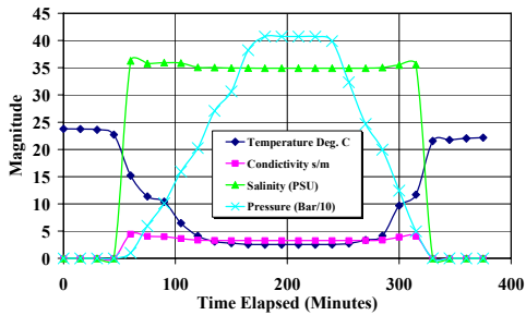
a – Internally Recorded CTD Data
