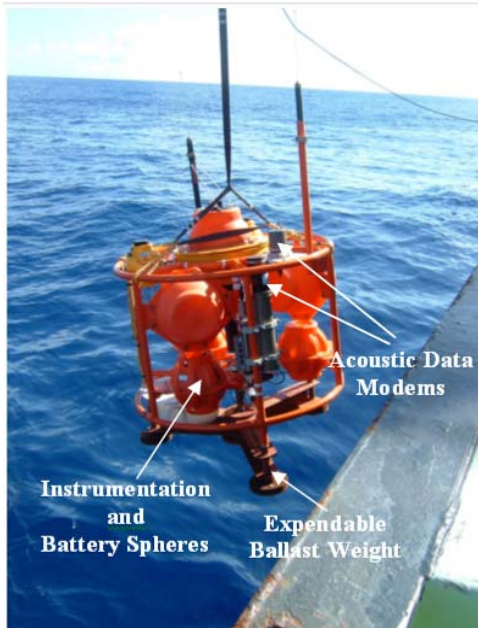
a – MYRTLE Upper View
