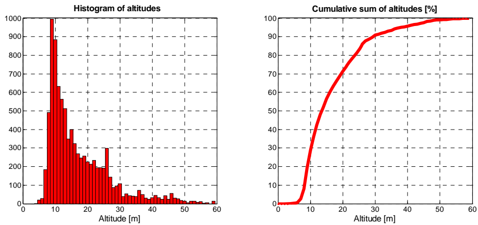
Figure 4. Statistical data during a 10m altitude terrain following ascent of the Casablanca Seamount.
