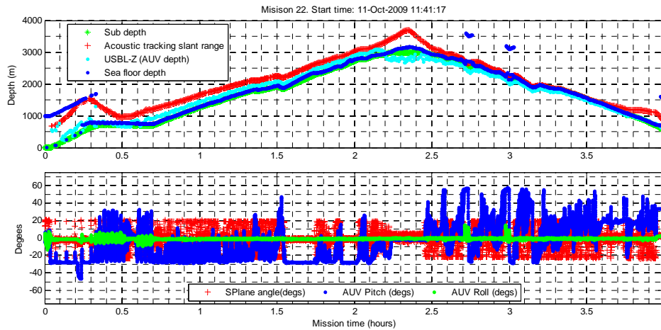
Figure 9. Mission 22. Low altitude (20m and 10m) demand transects across the Casablanca Seamount. Tracking and Telemetry worked reliably.
