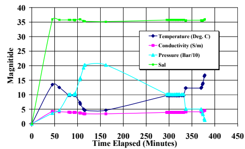
b – Received surface LinkQuest data that has been sampled and sent by the Orbcomm satellite global messaging service
