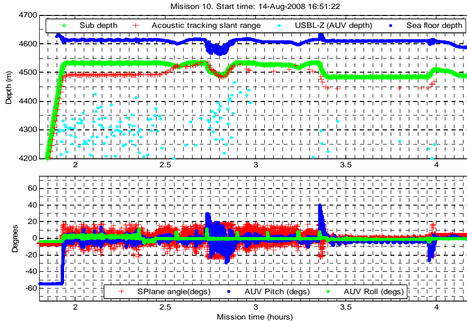
Figure 6. Mission 10 from the 2008 JC027 cruise. Red crosses in the top plot are Linkquest slant-ranges. Acoustic telemetry has been shown to reliably take place every time a slant range is received. Note how the slant range is received when the AUV is pitching, as indicated by the lower plot. Note also that the slant-range/telemetry is a response to a request message from the ship. If the ship is not transmitting then there will also be corresponding gaps in the plot data.
