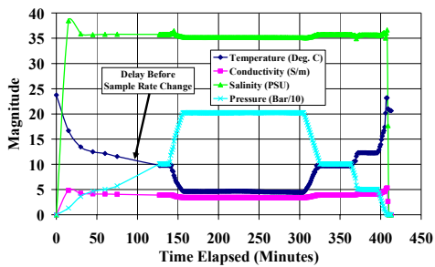
b – Internally recorded CTD Data
