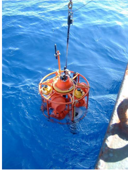
b – MYRTLE Deployment Just Prior to Release
