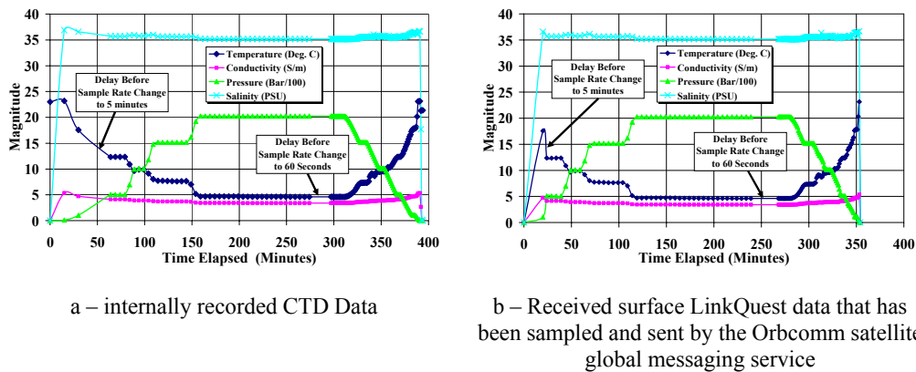
Fig. 10 – Recorded CTD and Telemetry Data from the Second 2000m Wire Test
