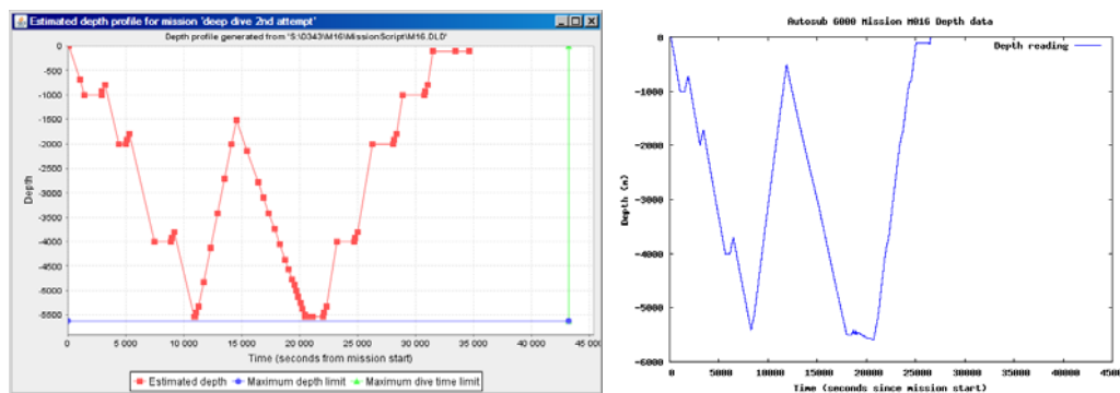
Figure 2 Comparison of predicted (left) and actual depth profile for Mission 16. The central peak of the graph was due to an error in the mission script.
