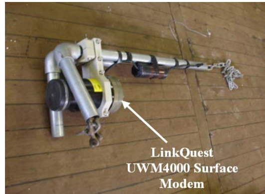
b – Assembled Surface Modem Mounting
