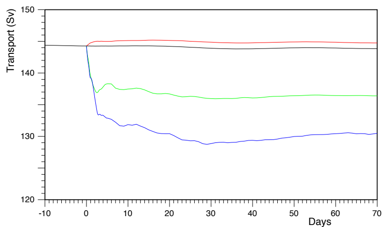
Fig. 2. Drake Passage transport during the analysis period. The lines are: Black – the control run; Red – perturbation run, zonal wind stress increased by 0.1 \text{ dyne cm}^{-2} at the latitudes of Drake Passage; Green – zonal wind stress set to zero at the same latitudes; Blue – wind stress set to zero everywhere. Days measured relative to day 3690 at the start of the analysis period. Transport in Sverdrups ( 1 \text{ Sv} = 10^6 \text{ m}^3 \text{ s}^{-1} ).
