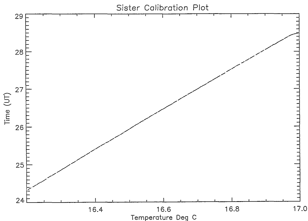
Figure 15.1 Graph showing a detail of the first SISTeR calibration. The SISTeR data are the dots, the actual temperature the line.
