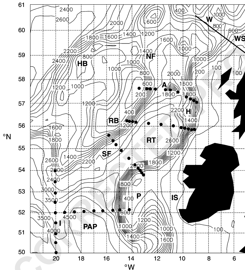
Fig. 1. Topography of the Rockall Trough and environs contoured from the model bathymetry (m), and selected CTD station positions (filled circles) from the “CHAOS” survey in May, 1998. Depth contours are shown at 100 m, every 200 m between 200 and 2600 m, 3000 m, and thereafter at 500 m intervals. The thick line between 60.6°N, 9°W and 59.1°N, 5°W represents the section across the Wyville–Thomson Ridge used for Fig. 6. The locations of the following features, referred to in the text, are also shown: Rockall Trough (RT); Rockall Bank (RB); Hatton Bank (HB); Wyville–Thomson Ridge (W); West Shetland Shelf (WS); Irish Shelf (IS); Hebrides Terrace Seamount (H); Anton Dohrn Seamount (A); Porcupine Bank (P); North and South Feni Ridge (NF and SF); Isengard Ridge (I); Porcupine Abyssal Plain (PAP).
