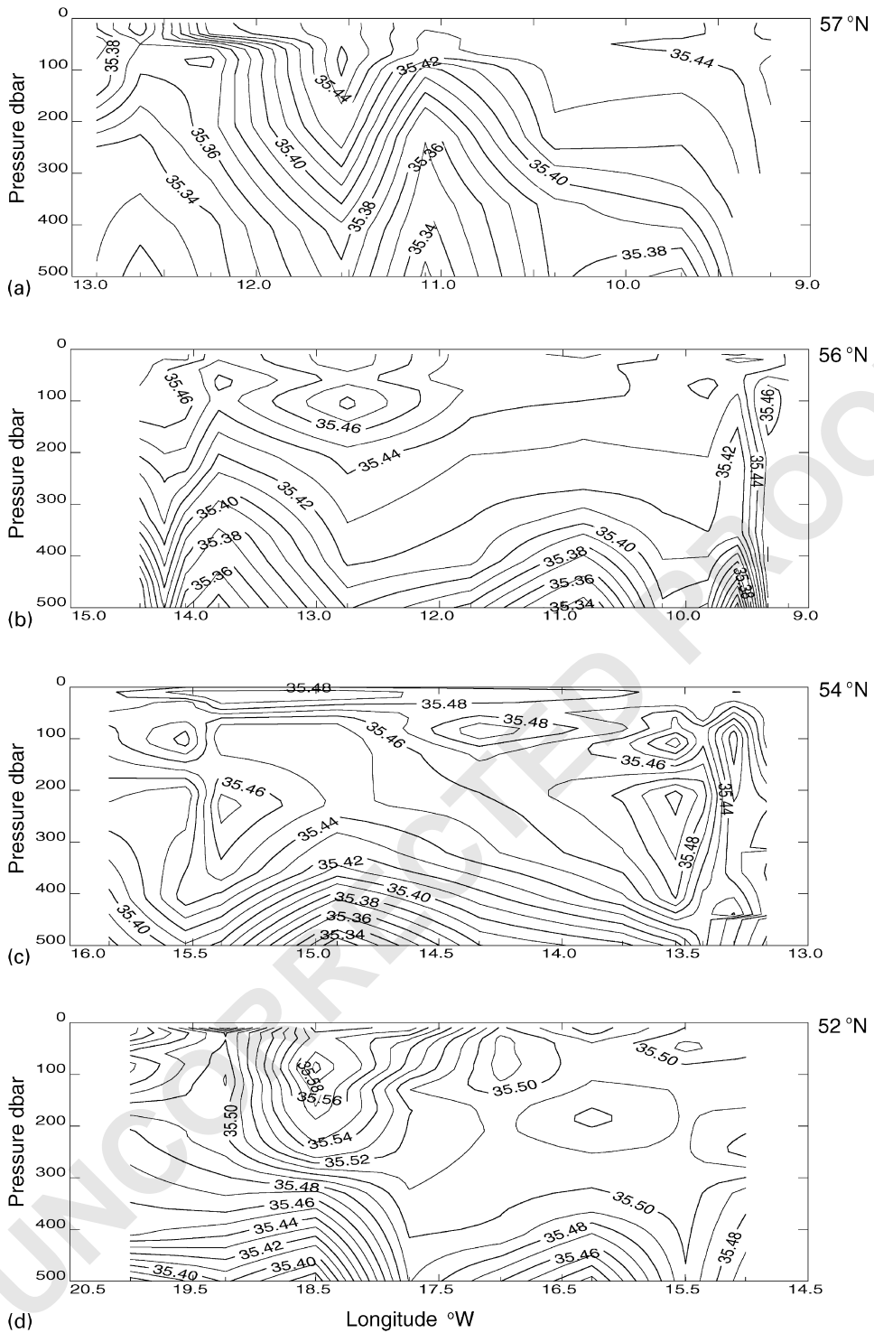
Fig. 3. Observed upper layer salinities along the sections (a) 57°N, (b) 56°N, (c) 54°N and (d) 52°N.
