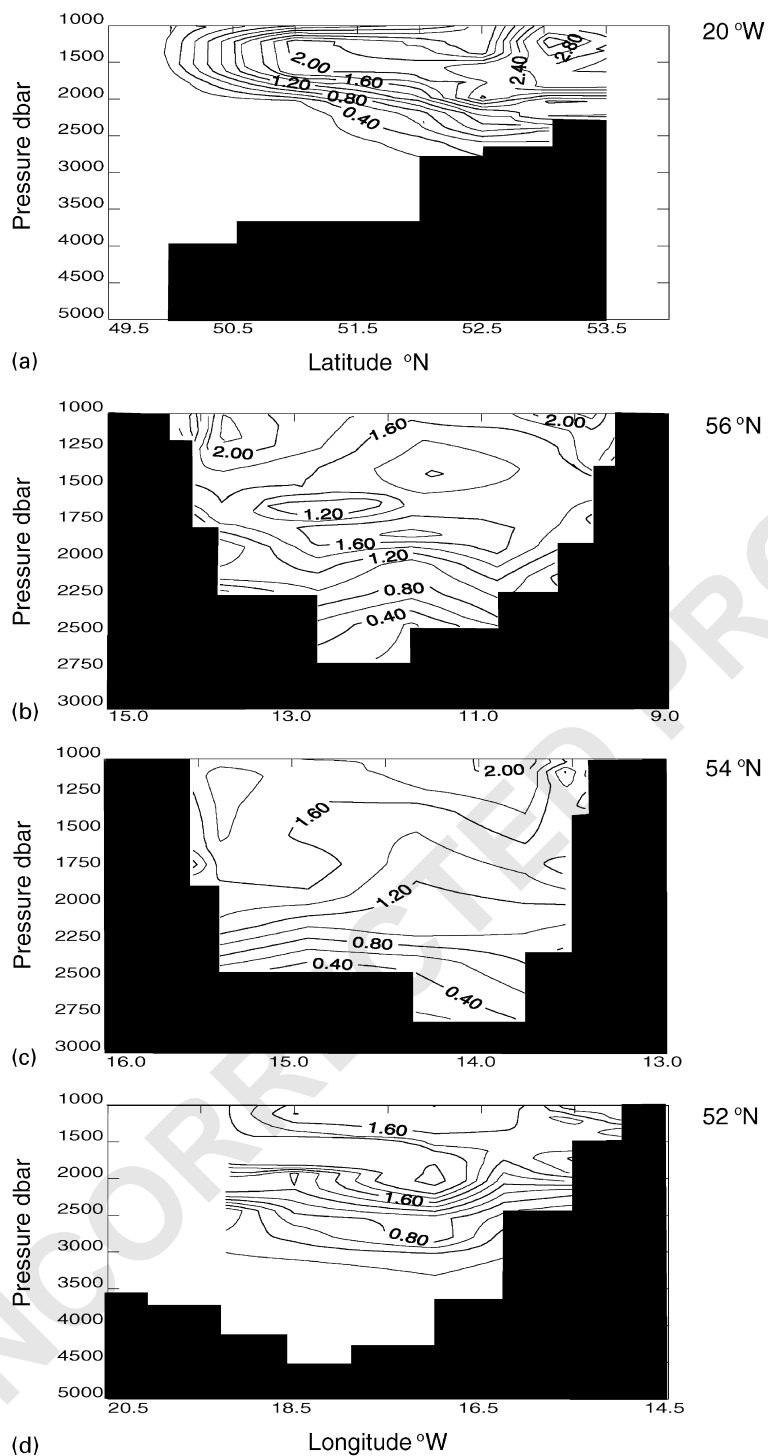
Fig. 9. Observed CFC-11 concentrations ( \text{p mol l}^{-1} ) below 1000 m depth on the sections (a) 20°W, (b) 56°N, (c) 54°N and (d) 52°N. Contours every 0.2 \text{ p mol l}^{-1} .
