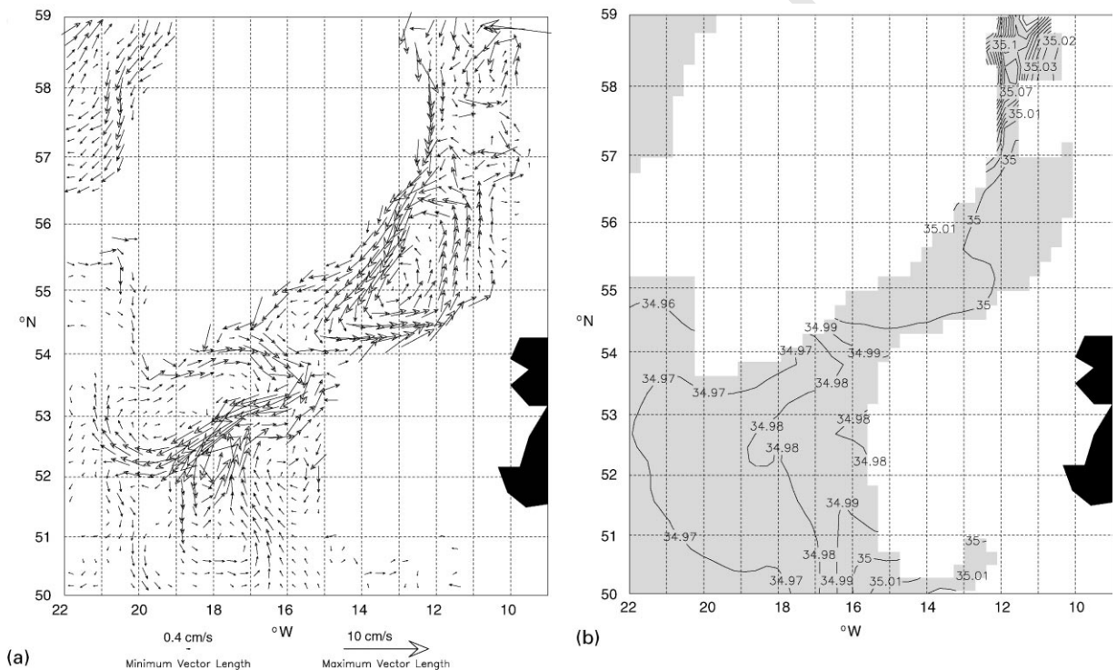
Fig. 7. Model structure on the Labrador Sea Water surface (corresponding to a density of 27.78). (a) Currents (cm s -1 ) and (b) salinity (contours every 0.01). In part (a), the vector arrows show the velocities at the arrow centres.
