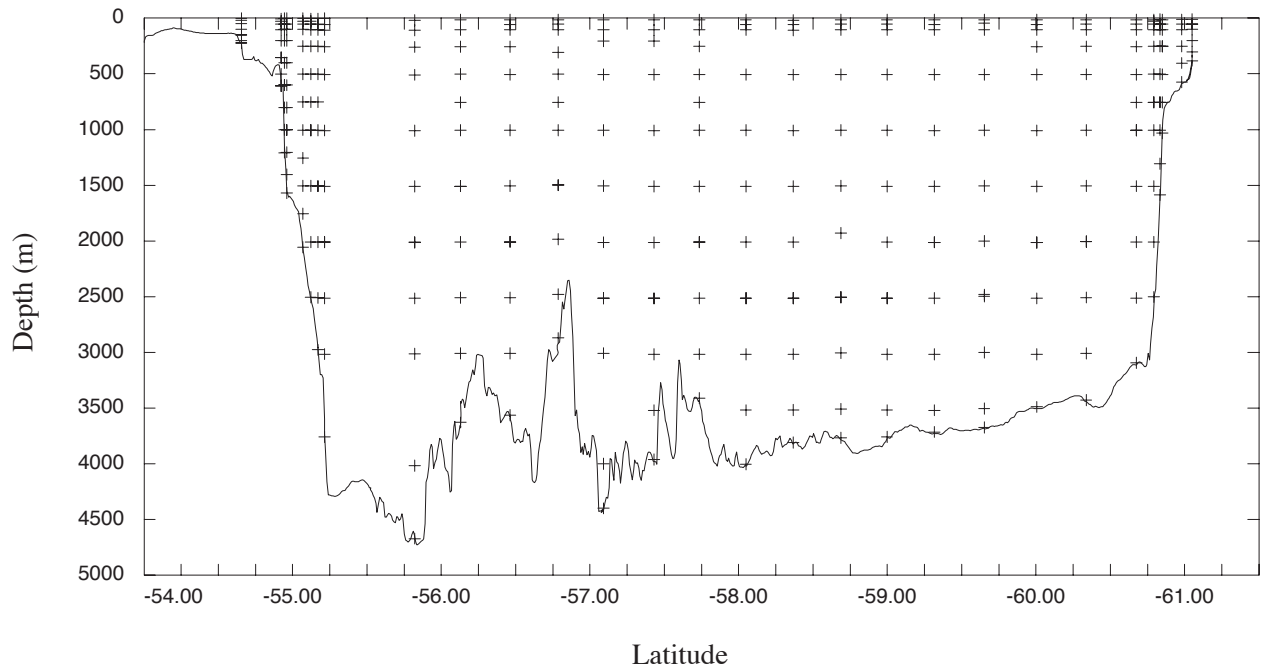
Figure 1.3: The bathymetry of the section across Drake Passage from the Simrad echosounder. Crosses (+) show the latitudes and depths of the bottle samples taken to calibrate the CTD conductivity sensors. Note the gap near the north end of the section where the CTD termination failed leading to no bottles being fired on station 10.
