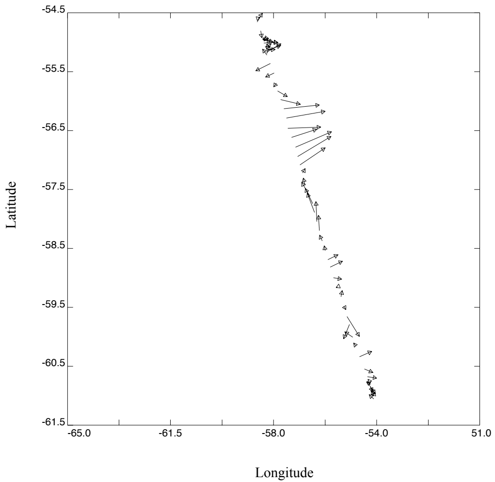
Figure 4.3: Vector plot of water track VM-ADCP data across Drake Passage SR1 section at a depth of 100 m, collected during JR67. Maximum vector magnitude 70.2 cm/s.
