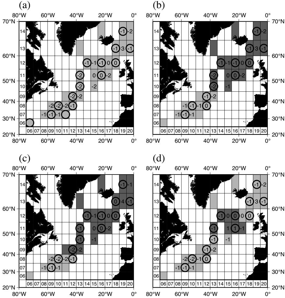
Fig. 8. Approximate nitrate residual \varepsilon_j(\mathcal{N}) ( \text{mmol m}^{-3} ) for (a) Calibration 1A, (b) Calibration 2A, (c) Calibration 2B and (d) Calibration 2C. Circled stations are the calibration stations used. The extent of each province is indicated by the shading.
