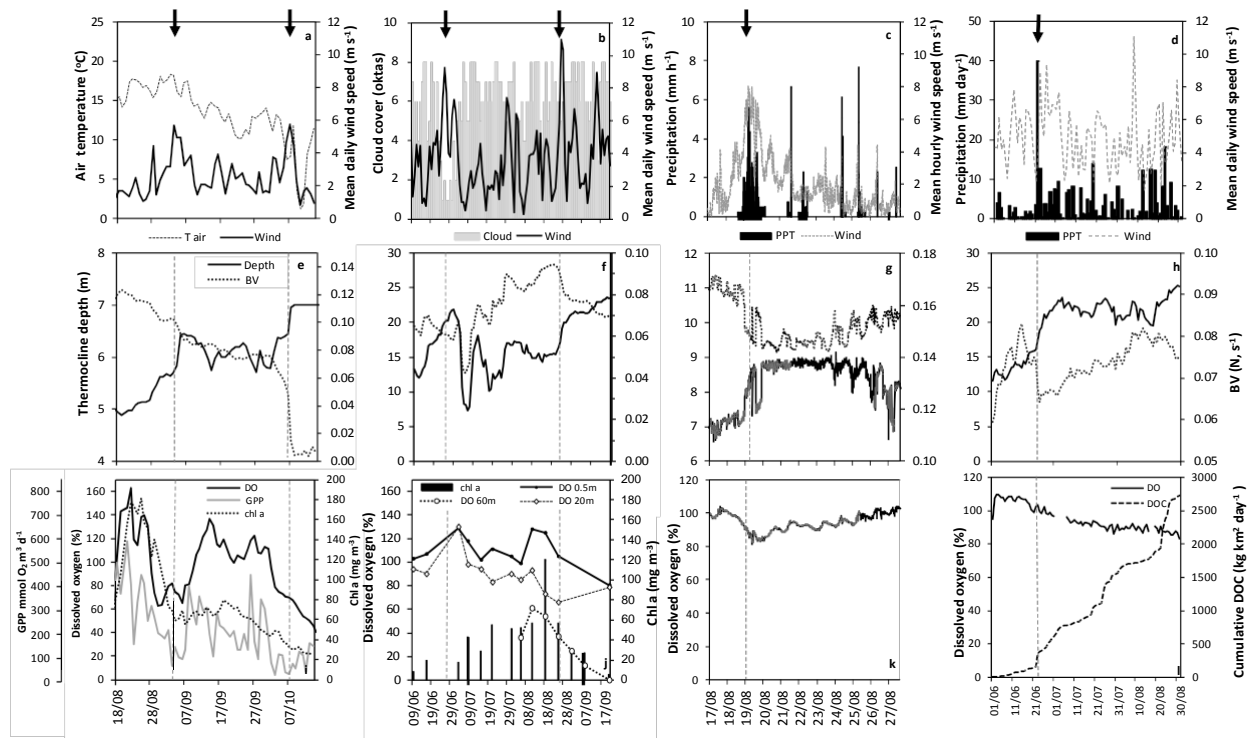
Fig. 2. Episodic events at Slotssø (a, e, i), Leane (b, f, j), Annie (c, g, k) and Feagh (d, h, l): meteorological drivers (a to d), Brunt Väisälä (BV) buoyancy frequency and thermocline depth (e to h), dissolved oxygen levels, chlorophyll a (Slotssø and Leane only) and gross primary productivity (Slotssø only), and inflow DOC load (Feagh only) (i to l). Black arrows and grey dashed lines indicate timing of change in meteorological driver.
