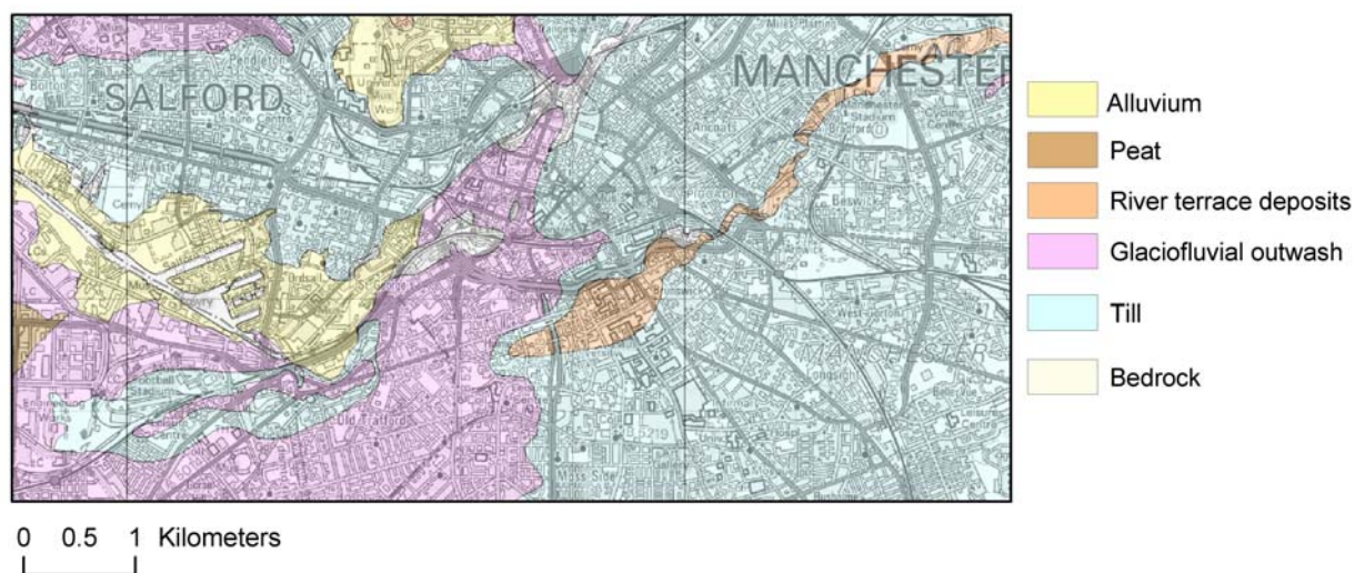
Superficial geology
