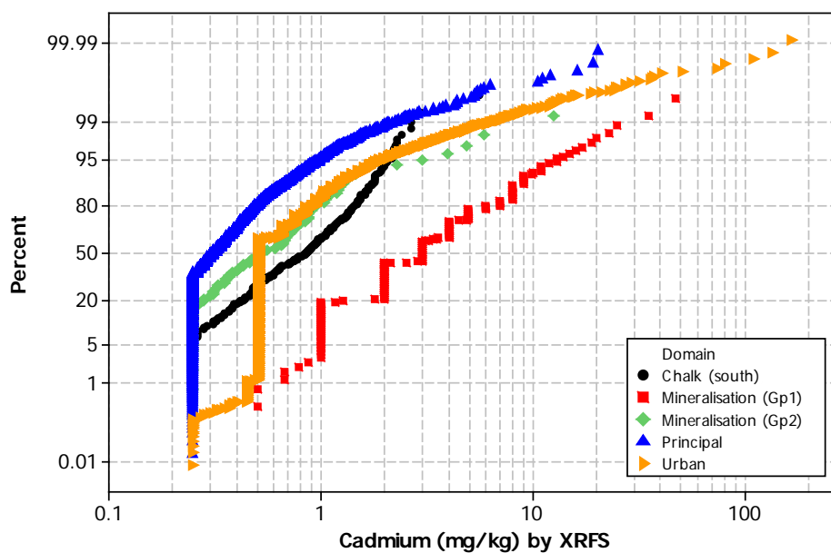
Figure 4: Probability plot of topsoil Cd results categorised by domains (Min. Gp1 is from the Peak District, Min. Gp 2 is from the N Pennines and Mendips).
