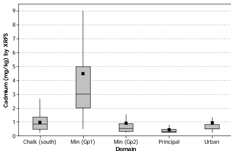
Figure 5: Boxplot of Cd topsoil results attributed to domains (Min. Gp1 is from the Peak District, Min. Gp 2 is from the N Pennines and Mendips).
