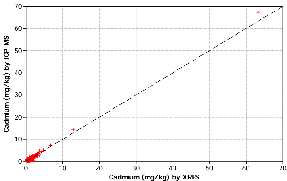
Figure 2: A comparison of topsoil Cd concentrations in Northern Ireland (Tellus Project) by XRFs and aqua regia digest ICP-MS
