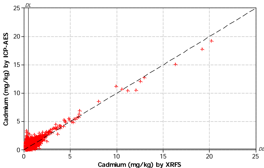
Figure 1: Comparison of topsoil Cd concentrations in NSI samples by XRFS and ICP-AES following aqua regia acid digest (DL is the detection limit)
