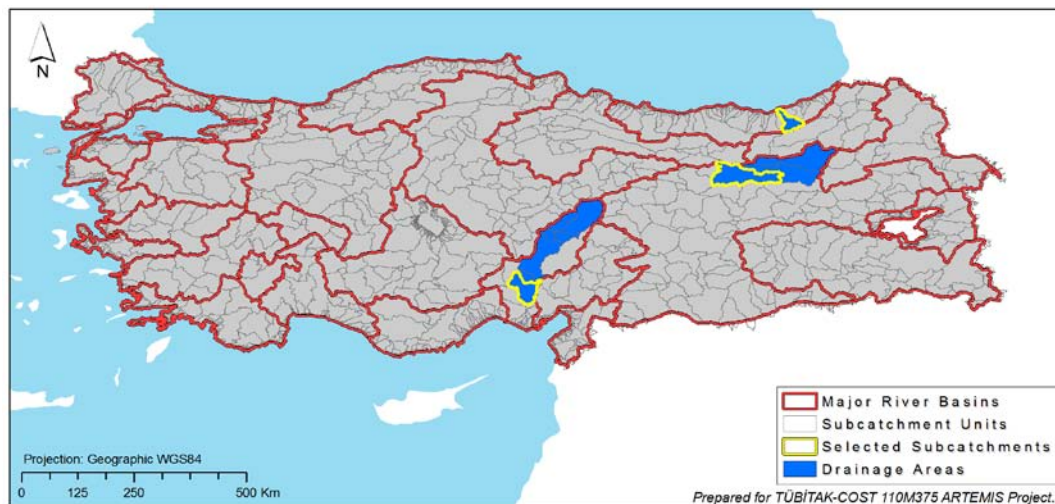
Figure TR2 Locations of pilot catchments identified for ARTEMIS Project, and pilot areas within Eastern BlackSea, Euphrates and Seyhan River Basins.
