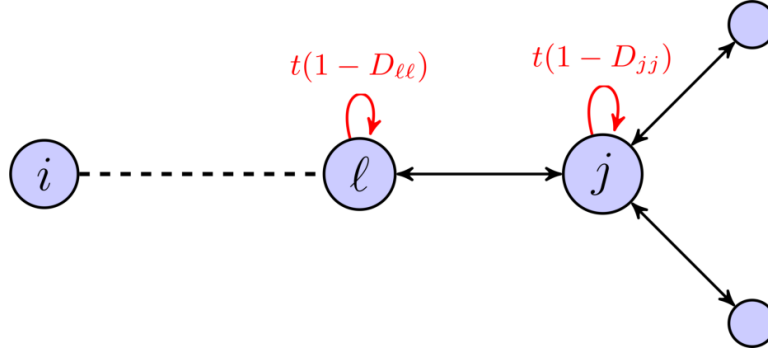
FIG. 2. Illustration of walks on the modified graph, for l \leftrightarrow j . In reaching node j via its neighbour l , an immediate backtrack to node l is eliminated by the loop at node l . Hence the continuation that finishes \ell j \ell j must be treated as a special case. Walks finishing \ell j h j for h \neq \ell are eliminated by the loop at node j .
