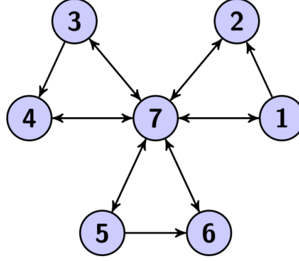
FIG. 1. Windmill network with m = 3 triangles.
