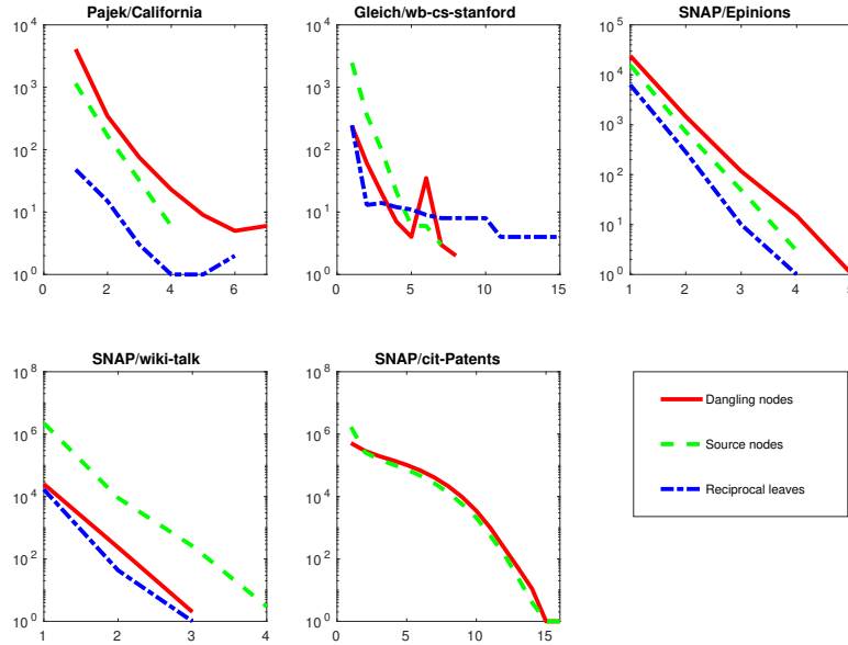
FIG. 8. Number of nodes removed at each step for each of the three types of nodes.
