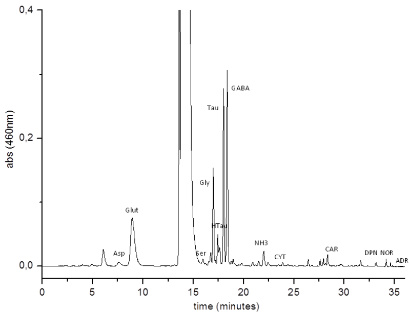
Fig. 8. HPLC chromatogram of dabsylated derivatives from neuroblastoma cell lysate
