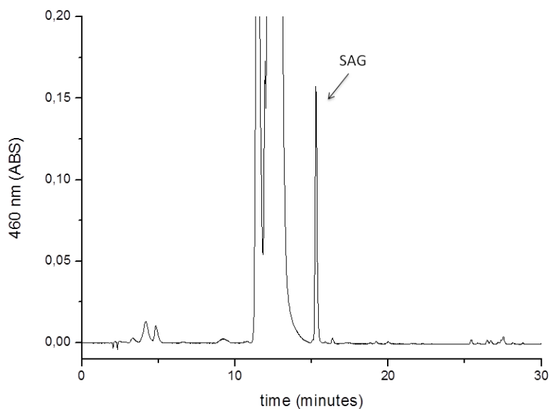
Fig. 10. HPLC chromatogram of dabsylated SAG
