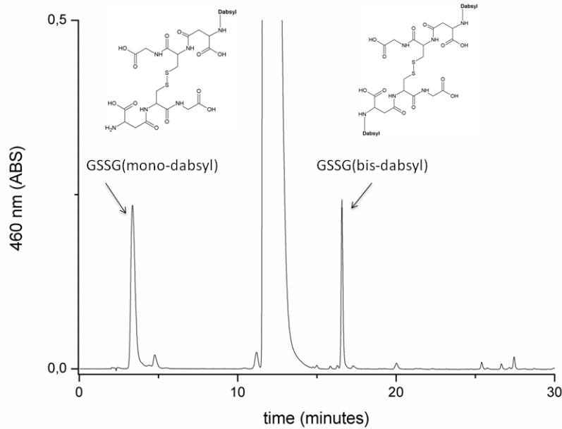
Fig. 11. HPLC chromatogram of Glutathione disulfide (GSSG)
