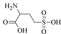
Homocysteic acid
