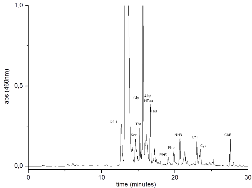
Fig. 6. HPLC chromatogram of dabsylated derivatives from human urine
