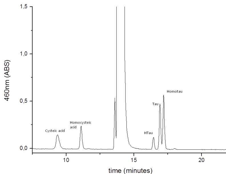
Fig. 12. HPLC chromatogram of Taurine and sulfur derivatives
