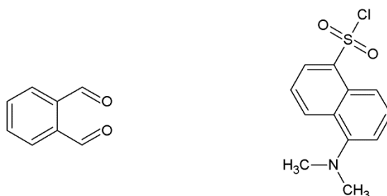
Fig. 3. Structures of OPA (left) and DANS (right)
