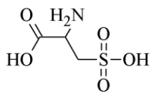
Cysteic acid
