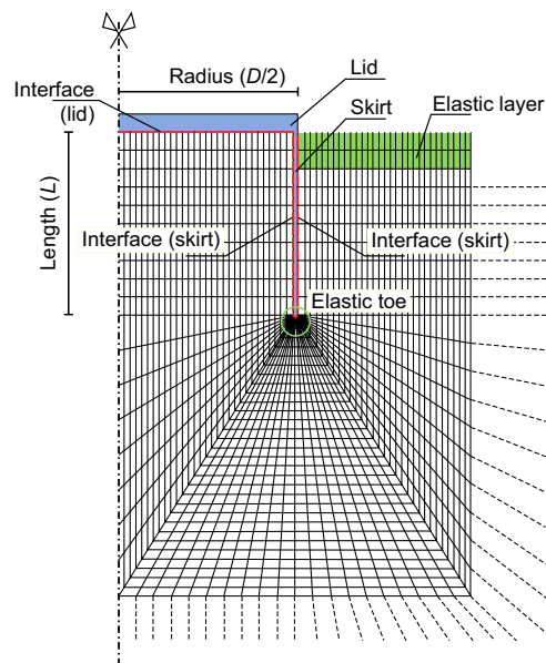
Fig. 2. Mesh adopted around the caisson
