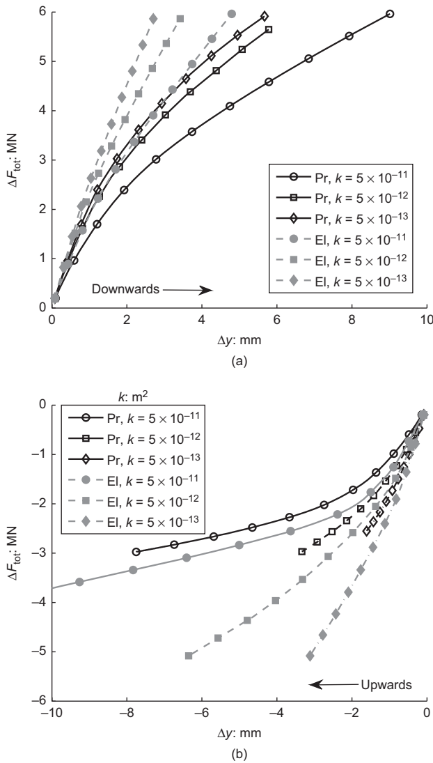
Fig. 14. Influence of the model (El for elastic linear or Pr for Prevost) and the permeability (three orders of magnitude, k = 5 \times 10^{-11} , 5 \times 10^{-12} , or 5 \times 10^{-13} \text{ m}^2 ) on partially drained results, pull rate 0.4 \text{ MN/s} : (a) compression simulation; (b) traction simulation
