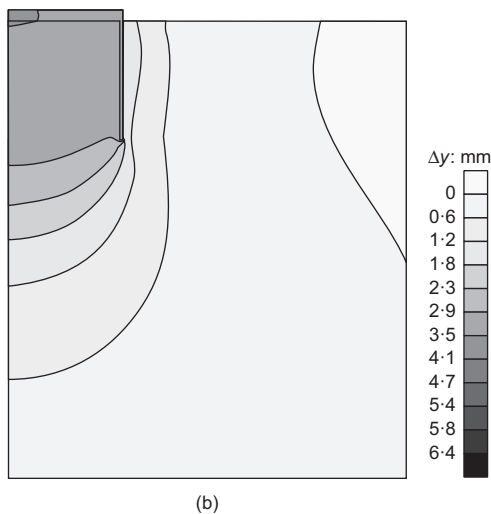
Fig. 10. Comparison of settlement of caisson and surrounding soil for \Delta F_{tot} = 4.3 MN
