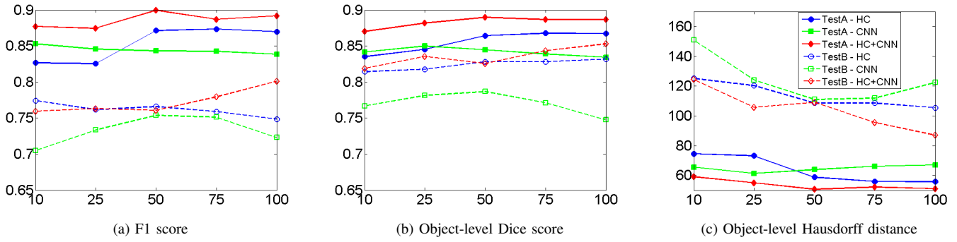
Fig. 7: Results (mean values) using structure prediction with different features and different values of K .
