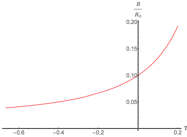
FIG. 1 (color online). The radius of low mass brown dwarf stars in alternative theories of gravity as a function of \Upsilon .
