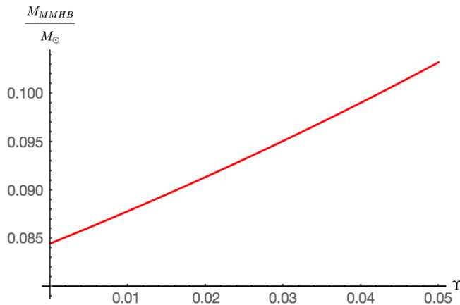
FIG. 2 (color online). The MMHB as a function of \Upsilon .
