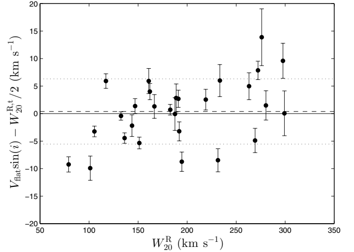
Fig. 3. Difference between the weighted-average, projected rotational velocities of the H \alpha , [OIII] and HI PV diagrams and half the corrected widths of the HI global profiles. The dashed line shows the average difference while the rms scatter is indicated by the two dotted lines.
