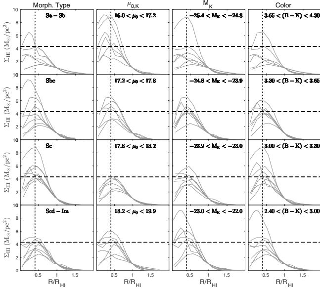
Fig. 8. Compilation of all 28 HI column density profiles, divided in four non-equal bins for each of four global optical properties; morphological type, central disk surface brightness, absolute magnitude, and color. The profiles are scaled in radius by R_{\text{HI}} . The horizontal dashed lines are drawn at the sample median \Sigma_{\text{HI}}^{\text{max}} of 4.3 \text{ M}_{\odot} \text{ pc}^{-2} as a reference. The vertical dotted lines are drawn at the radius where the average profile reaches its peak column density.
