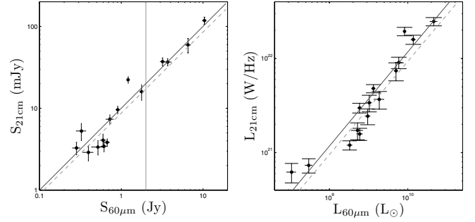
Fig. 14. Radio-infrared correlation of 15 galaxies in the reduced HI sample detected by IRAS at 60\ \mu\text{m} . Left: correlation between flux densities. The solid line indicates the simple relation S_{21\text{ cm}} = 0.01S_{60\ \mu\text{m}} . The dashed line shows the correlation found by Yun et al. (2001) for the IRAS 2 Jy sample. The vertical line indicates their lower flux-density limit of 2 Jy. Right: correlation between intrinsic radio and infrared luminosities.
