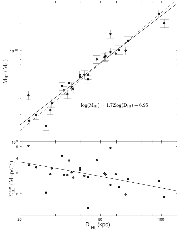
Fig. 6. Upper panel: correlation between the total HI mass ( M_{\text{HI}} ) and the beam-corrected diameter of the HI disk ( D_{\text{HI}} = 2R_{\text{HI}} ). The solid line shows the fit to the data while the dashed line represents the correlation found by Verheijen & Sancisi (2001). Lower panel: average HI mass surface density within R_{\text{HI}} versus D_{\text{HI}} . The line indicates the expected slope based on the fit in the upper panel .
