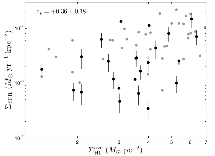
Fig. 16. Star formation density versus average HI mass surface density for the galaxies in our sample (black) and the galaxies in Kennicutt (1998; gray).
