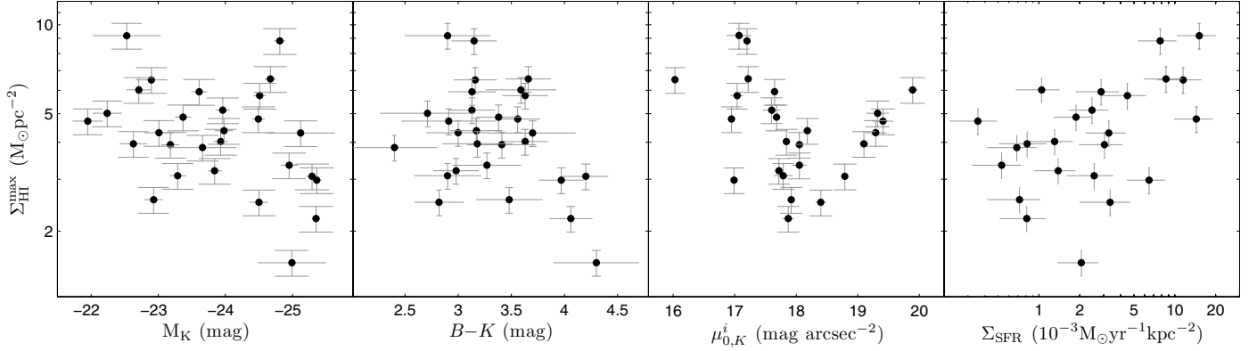
Fig. 9. Relations between the maximum, azimuthally-averaged HI column densities ( \Sigma_{\text{HI}}^{\text{max}} ) and global properties of the galaxies. From left to right: absolute K -band magnitude, B - K color, central disk surface brightness, and star formation density.
