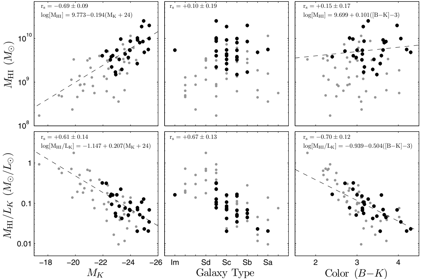
Fig. 5. Total and relative HI masses as a function of M_K (left), morphological type (middle), and B-K color (right). The dashed lines are fits to the DMS galaxies (black symbols). The gray symbols show the galaxies from Verheijen & Sancisi (2001).
