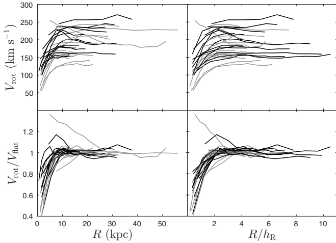
Fig. 11. Compilation of all 28 derived rotation curves with different scalings for each panel. The sample of rotation curves is divided in two according to central disk surface brightness: gray curves correspond to galaxies of lower surface brightness ( \mu_{0,K}^i > 17.8 \text{ mag/arcsec}^2 ) and black curves correspond to galaxies of higher surface brightness ( \mu_{0,K}^i < 17.8 \text{ mag/arcsec}^2 ). In the upper left panel, no scaling is applied to the rotation curves. In the bottom right panel, the rotation curves are scaled both in radius and amplitude.
