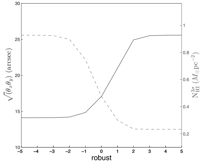
Fig. 1. Illustration of the trade-off between angular resolution and column-density sensitivity for different robust weightings of the WSRT visibility data, ranging from uniform to natural weighting. The solid curve indicates the size of the synthesized beam, and the dashed curve shows the 3\sigma column-density sensitivity in a single channel.
