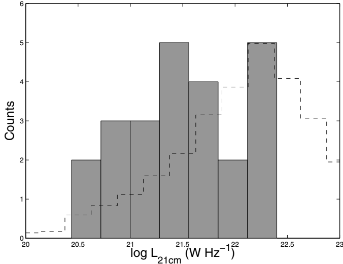
Fig. 13. Distribution of 21 cm radio continuum luminosities. The solid histogram displays the distribution of 21 cm radio continuum luminosities of the galaxies in the reduced HI sample. The dashed histogram shows the distribution for the IRAS galaxies as derived by Yun et al. (2001).
