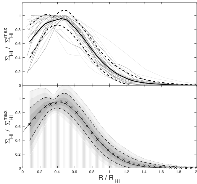
Fig. 10. Self-similarity of the HI column density profiles. Upper panel: all 28 \Sigma_{\text{HI}} profiles scaled in radius and normalized in amplitude. The thinnest lines correspond to the early-type spirals in our sample. The thick black line shows the clipped average profile and the dashed lines indicate the rms scatter at each radius. Lower panel: the crosses follow the thick black line in the upper panel and the dashed lines are identical to the dashed lines in the upper panel. Gray scales indicate steps of 0.5 times the rms scatter. The solid black line is the best-fit Gaussian function following the crosses above (\Sigma_{\text{HI}}/\Sigma_{\text{HI}}^{\text{max}}) > 0.2 .
