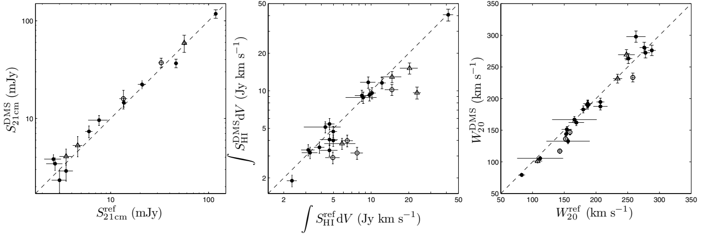
Fig. 2. Comparison of our measurements with data from the literature. Left: total 21 cm radio continuum flux densities. Middle: integrated HI line fluxes. Right: HI line widths at the 20% level of peak intensity. Solid symbols represent data from the WSRT, open circles from the VLA, and open triangles from the GMRT. The data are listed in Table 3 with references to the literature values.
