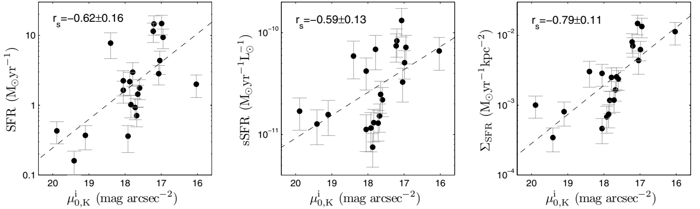
Fig. 15. Relations between disk surface brightness ( \mu_{0,K}^i ) and total SFR ( left ), specific SFR ( middle ), and SFR surface density ( right ). The dashed lines are linear fits to the data.
