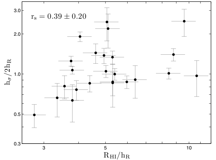
Fig. 7. Comparison of the relative kinematic scale lengths of the stellar disks and the relative size of the HI disks. Galaxies in which the stellar velocity dispersion decreases faster with radius than expected on the basis of the photometric scale length of the stellar disk ( h_{\sigma}/2h_R < 1 ), tend to have relatively small HI disks, and vice versa.
