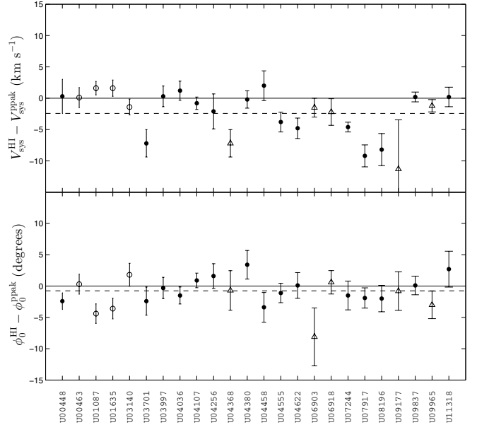
Fig. 4. Comparison of results from HI observations with those from optical PPAk observations. The figure shows differences between the systemic velocities ( upper panel ) and between position angles of the kinematic major axis in the inner regions of the galaxies ( lower panel ), measured from the HI velocity fields and those measured with the PPAk IFU from [OIII] and stellar velocity fields (Paper VI). The dashed horizontal lines show the average differences. Solid points correspond to WSRT data, open circles to VLA data, and open triangles to GMRT data.
