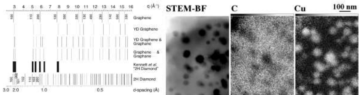
Figure 1. Left: Predicted electron diffraction of 2H diamond (with both general and special extinctions), graphene, and graphene/graphane mixture. Shown also are those from graphene and graphene/graphane aggregates in YDB carbon spherules as well as those identified as 2H diamond (line widths represent error in our measurement of diffraction patterns reported in [3]), all from Santa Rosa Island, CA. Right: Native Cu nanocrystals in YDB carbon spherules (i.e., sclerotia [9]) from Santa Rosa Island, CA (gray scale LUT of STEM-EDXS elemental maps: black = minimum, white = maximum).
