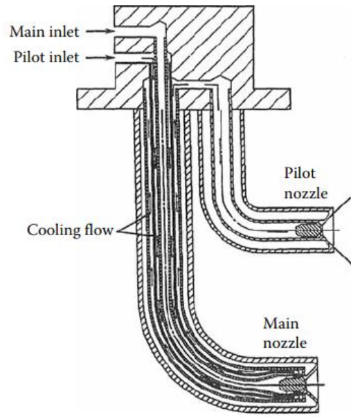
Figure 14. GE-DAC Twin-tip fuel injector with main nozzle cooled by the pilot fuel flowing around it to provide effective cooling [9]
