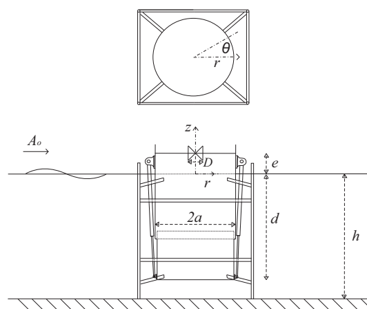
Fig. 1 Sketch of the OWC system [8]
