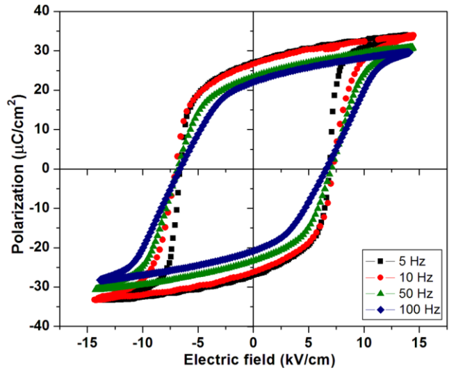
Fig. 7. P - E loops measured at frequencies of 5, 10, 50 and 100 Hz of an unfatigued sample.
