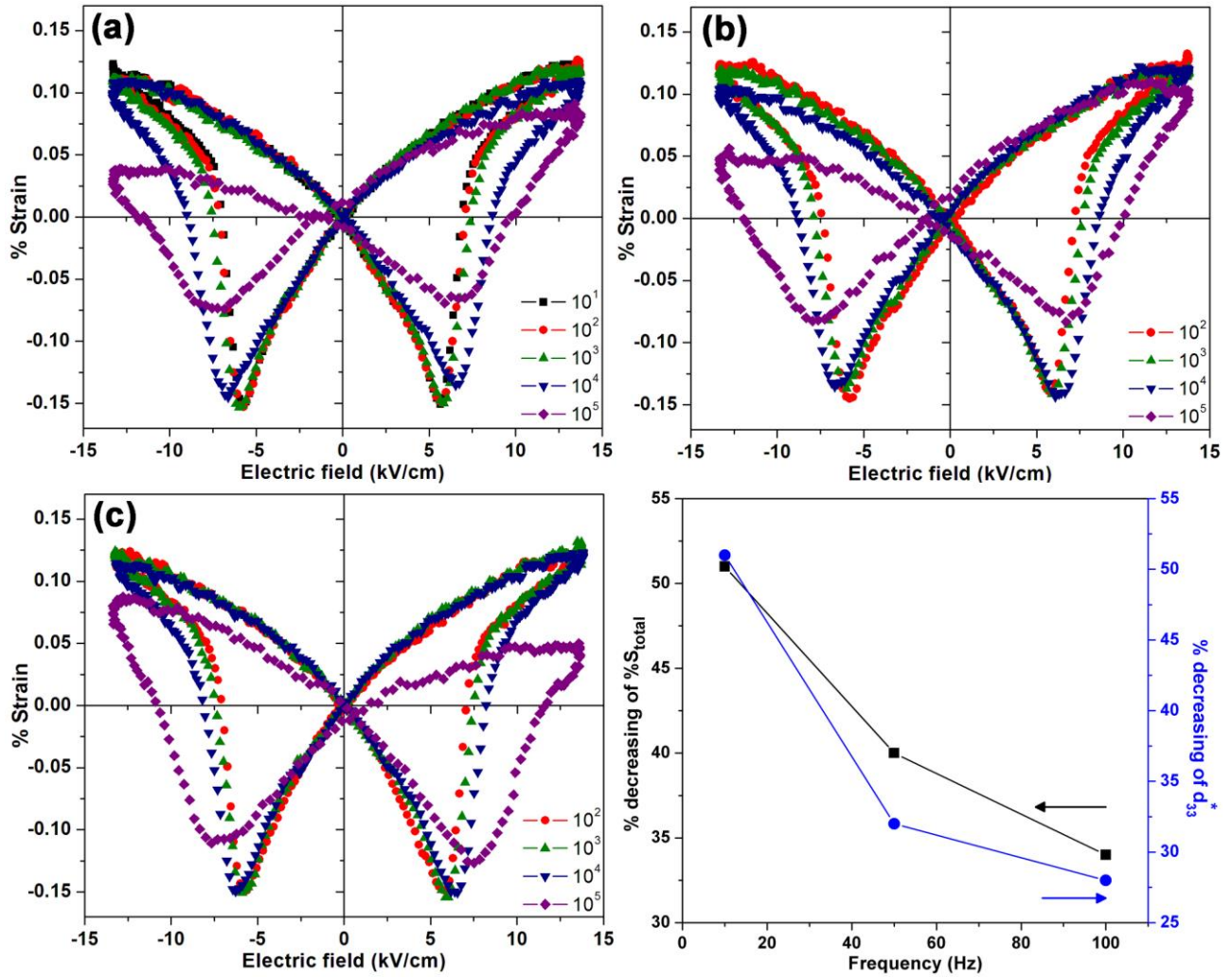
Fig. 6. % Strain versus electric field loops measured at different cycle numbers of the samples fatigued at (a) 10, (b) 50 and (c) 100 Hz. (d) Plots of percent decrease in \%S_{total} and d_{33}^* as a function of fatigue frequencies of ZnO-modified PMNT ceramics.
