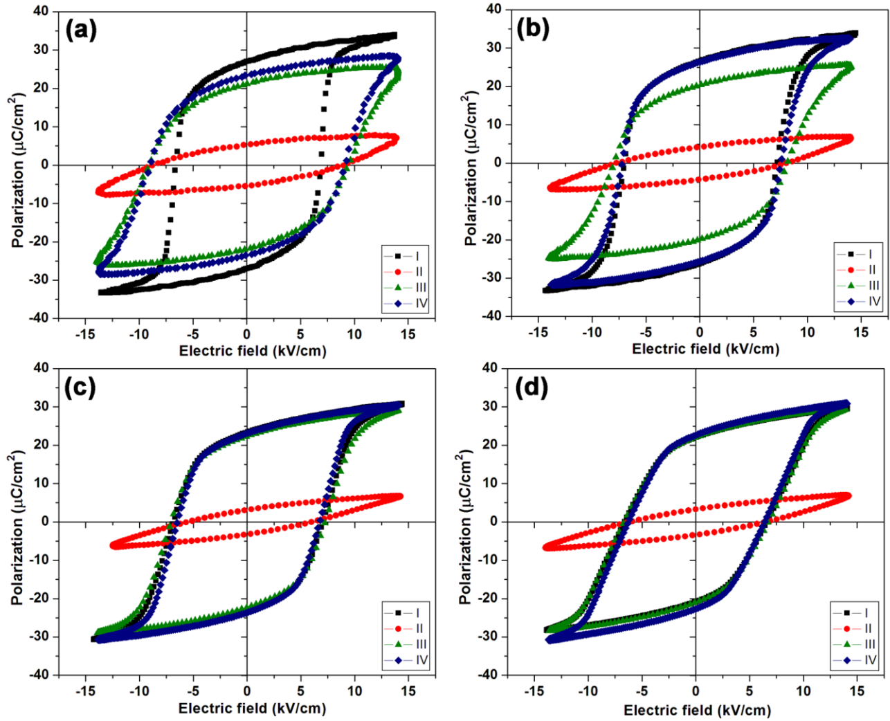
Fig. 4. P - E loops measured (I) before fatigue test, (II) at 10^6 cycles fatigue test, (III) after removing the damaged layers and (IV) after annealing at 500\text{ }^\circ\text{C} for 2 hrs of the samples fatigued at (a) 5, (b) 10, (c) 50 and (d) 100 Hz.
