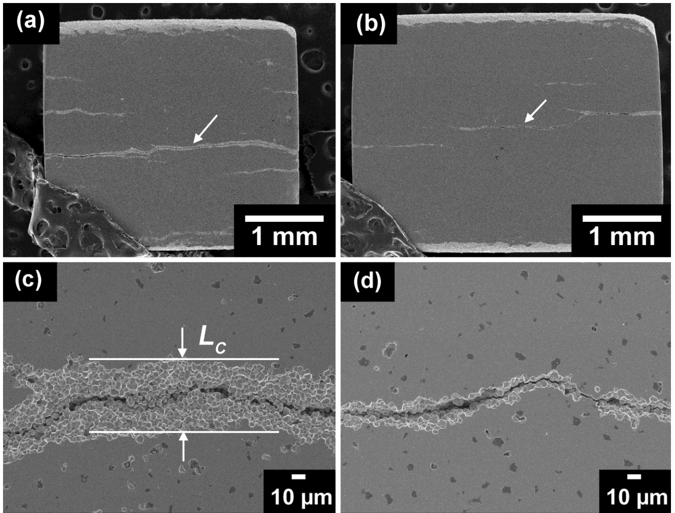
Fig. 2. SEM images of mirror-like surfaces of samples fatigued for 10^6 cycles at (a) 5 and (b) 10 Hz. Electric field induced-cracks are indicated by the arrows. Enlarged views of a crack observed in samples fatigued at 5 and 10 Hz are shown in (c) and (d), respectively. Crack width is denoted as L_c .
