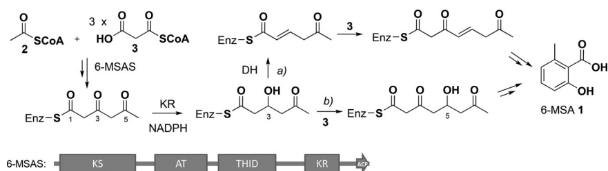
Scheme 1. Overview of biosynthetic hypotheses leading to 6-methylsalicylic acid (6-MSA, 1 ): a) enzymatic dehydration of a 3-hydroxytriketide followed by further chain extension leads to a dehydrated enzyme-bound tetraketide, eventually giving 1 ; b) formation of a 5-hydroxytetraketide eventually leading to 1 via TH-mediated hydrolysis. [18c,19b] 6-MSAS comprises ketosynthase (KS), acyltransferase (AT), thioester hydrolase (THID), [19b] ketoreductase (KR), and acyl carrier protein (ACP) domains.
