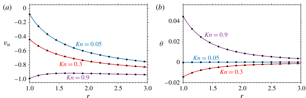
FIGURE 3. The polar velocity v_\alpha at \alpha = \pi/2 and temperature \theta at \alpha = 0 for flow around a sphere. The R13-MFS predictions ( \bullet , \blacktriangle , \blacksquare ) for Kn = 0.05, 0.3, 0.9 respectively compared with the analytic result from Torrilhon (2010) (solid lines).
