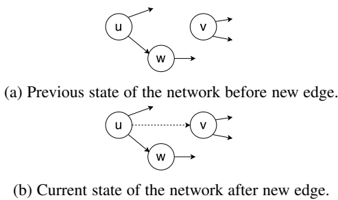
Fig. 3: A sample network for analysis.
