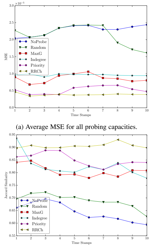
Fig. 12: Comparison of the Probing strategies with respect to time.
