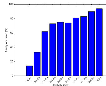
Fig. 14: Accuracy of the link prediction algorithm.
