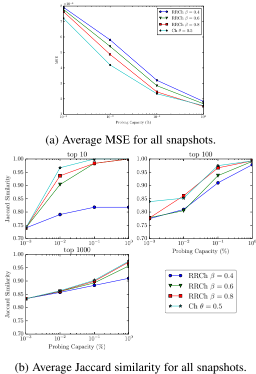
Fig. 8: Performance of RRCh w.r.t. \beta .
