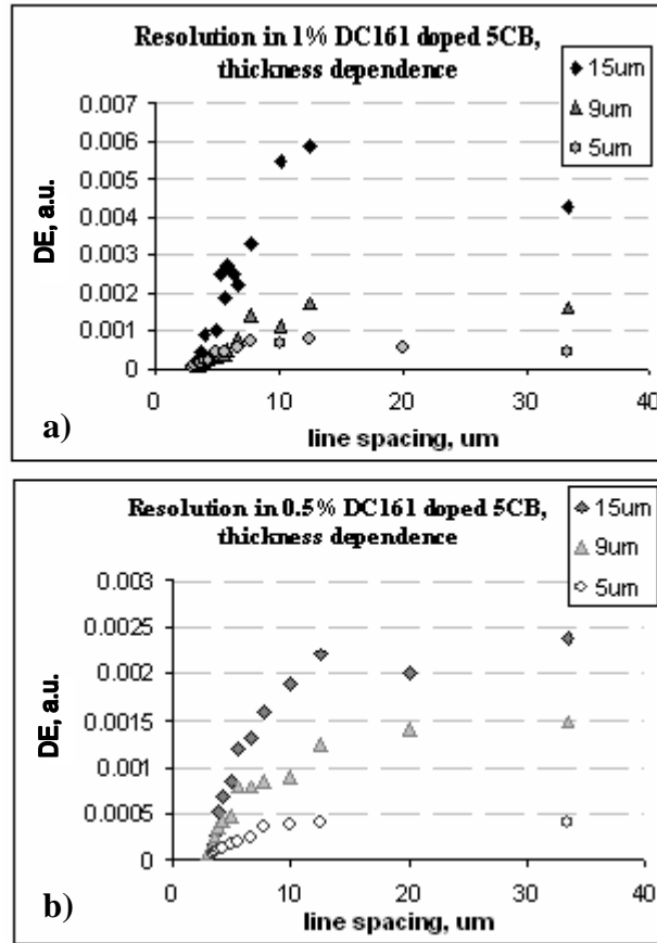
Fig. 3. Diffraction efficiency (in arbitrary units) versus the period of the grating ( in \mu\text{m} ): for 1% wt (a) and 0.5% wt (b) dye concentrations; sample thickness as parameter.
