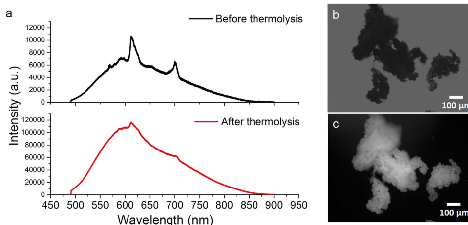
Figure 6. (a) Solid state photoluminescence spectra of compound 1 before (black) and after (red) thermolytic treatment, (b) bright field and (c) fluorescence ( \lambda_{\text{ex}} 365 nm) microscope images of compound 1 following thermolysis.
