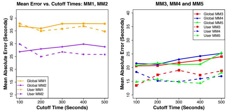
Figure 3: The mean absolute error of the predictions for each Markov chain model over the cutoff times (refer to Section 4). Note that the absolute error is compared over the various interaction data cutoff times.
