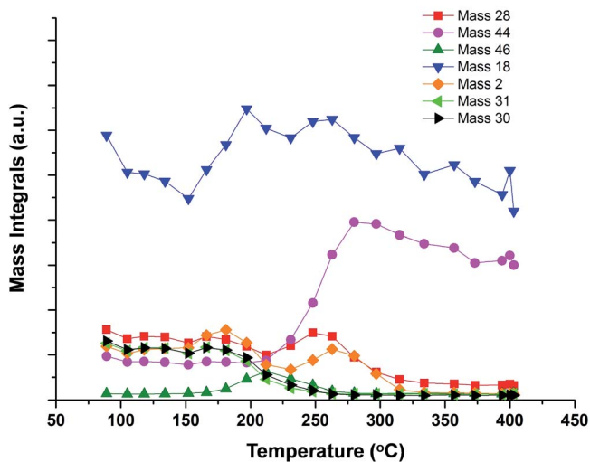
Fig. 7 TPR (temperature-programmed pulse reaction) profiles for methanol pulses into a flow of He.
