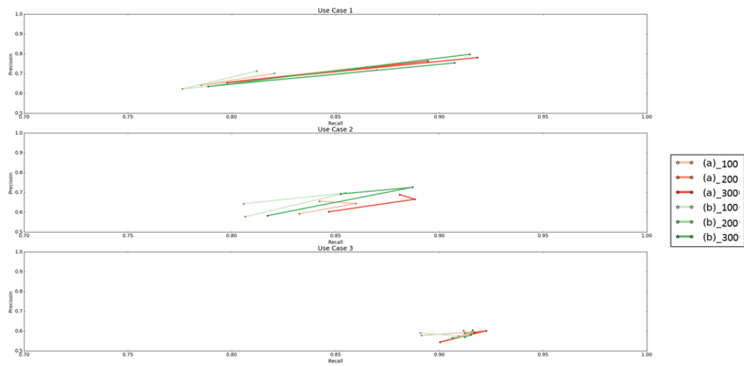
Figure 5. A comparison of precision/recall rates for raster sampling method (a) and (b) with an adjustment of cell sized from 0.00091 decimal degrees under WGS_1984 to one and half and double size (approximately 60, 85 and 110 meters).
