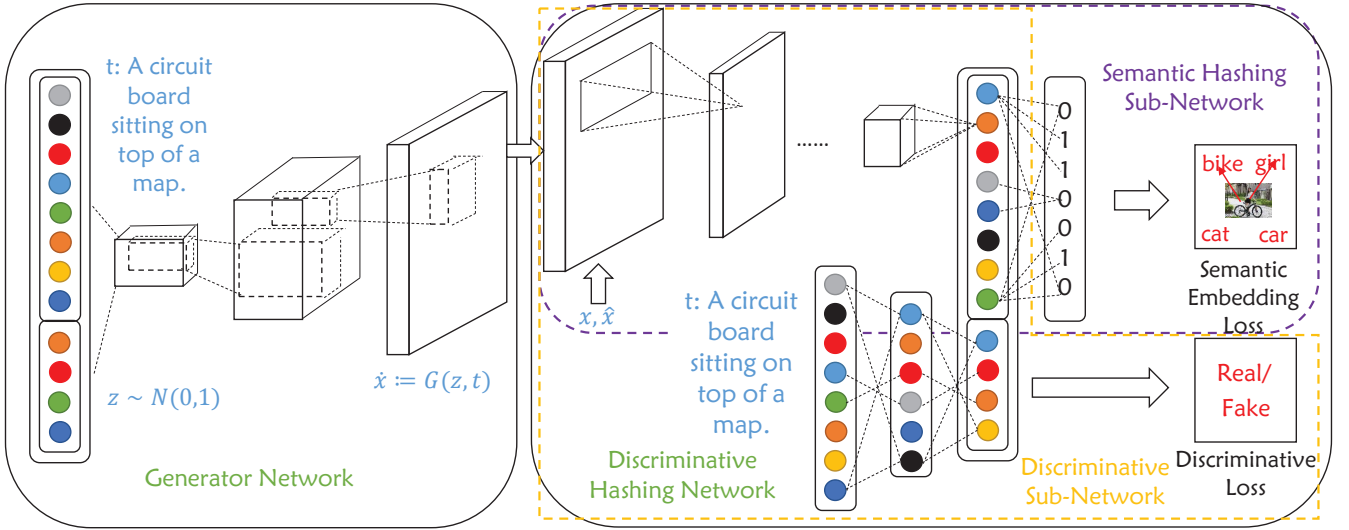
Figure 2: Our multi-task TUCH architecture. Generator network and discriminative sub-network constitute a normal conditional GANs. Semantic hashing sub-network is a normal image hashing network based on CNN. Text encoding t extracted by language model T is used in both generator network and discriminative hashing network. x is real relevant image, \hat{x} is fake image generated by G with t, \hat{x} is real irrelevant image.
