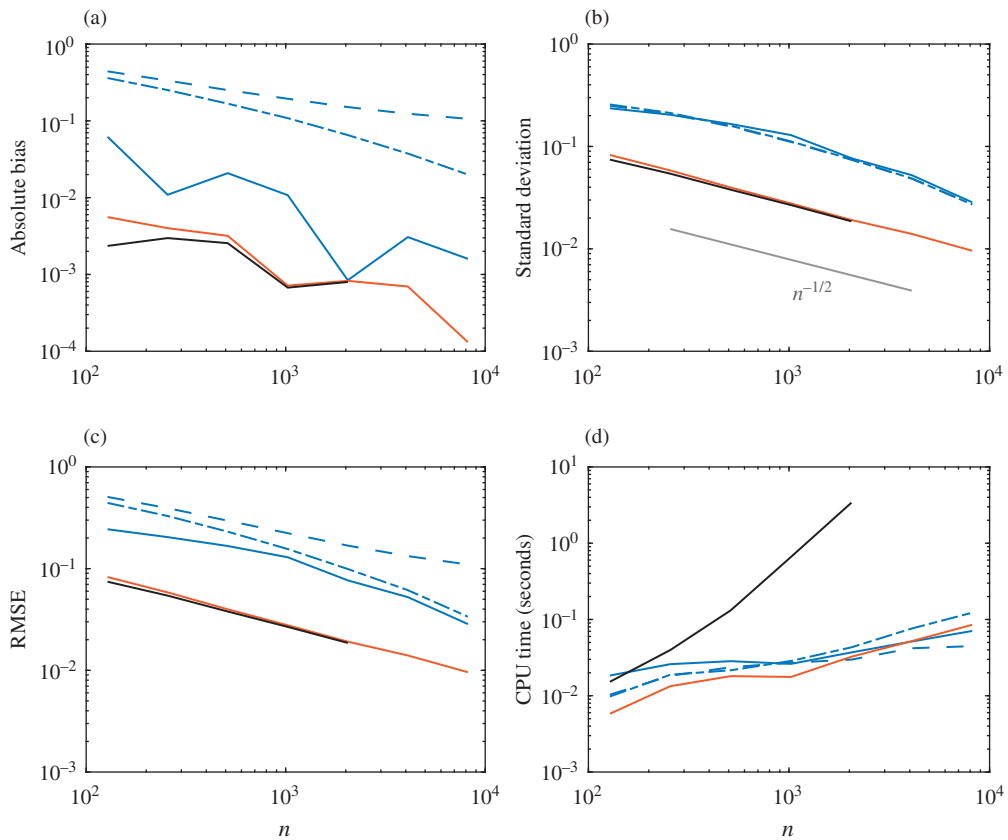
Fig. 1. Performance in terms of (a) absolute bias, (b) standard deviation, (c) root mean square error, and (d) CPU time of five different likelihoods: standard Whittle unaliated (blue dashed); standard Whittle aliased (blue dot-dashed); debiased Whittle periodogram (blue solid); debiased Whittle differenced (red solid); and exact maximum likelihood (black solid). Results were obtained over 1000 repetitions for various values of n when estimating the slope parameter ( \alpha = 2 ) of a Matérn process. The axes are on a log-log scale, and CPU times are for computations performed on a 2.2 GHz Intel Core i7 processor.
