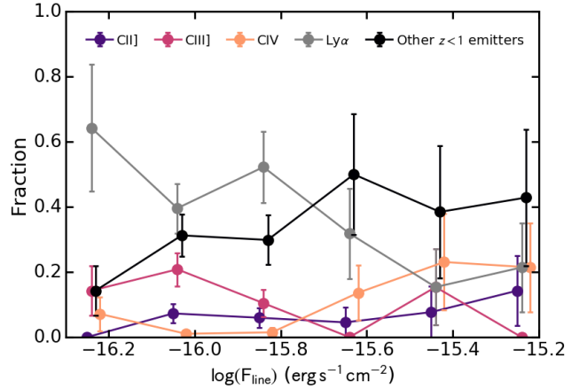
Figure 2. The fraction of CII], CIII], CIV and \text{Ly}\alpha emitters as function of line flux, derived using sources with redshifts, down to an observed EW limit of 16 \text{ \AA} . Note the decreasing fraction of \text{Ly}\alpha emitters at the largest fluxes, where the population is comprised of \sim 40 per cent CIII] and CIV emitters. We also overplot the fraction of lower redshift ( z < 1 ) emitters such as [OII], NeV, MgI and MgII. Note that some of these might still be CII] or CIII] emitters, given our conservative photometric redshift ranges (see for example, Fig. 2 in Stroe et al. 2017a).
