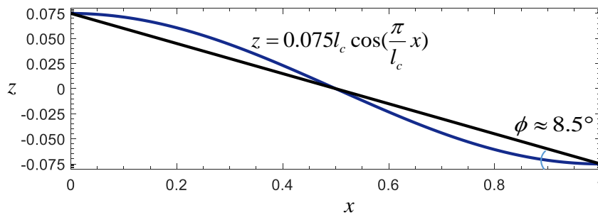
Fig.4. A cosine-type curve cantilever beam and an inclined straight cantilever beam with an angle of 8.5^\circ with respect to the x - y plane. Their lengths are close to l_c , with the former at 1.0137l_c and the latter at 1.0111l_c . The x and z axes are normalized by l_c .
