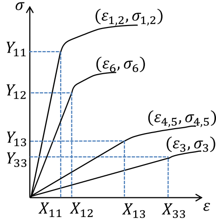
Fig.7. The elastic-plastic response of transversely isotropic materials under uniaxial loading and pure shearing.
