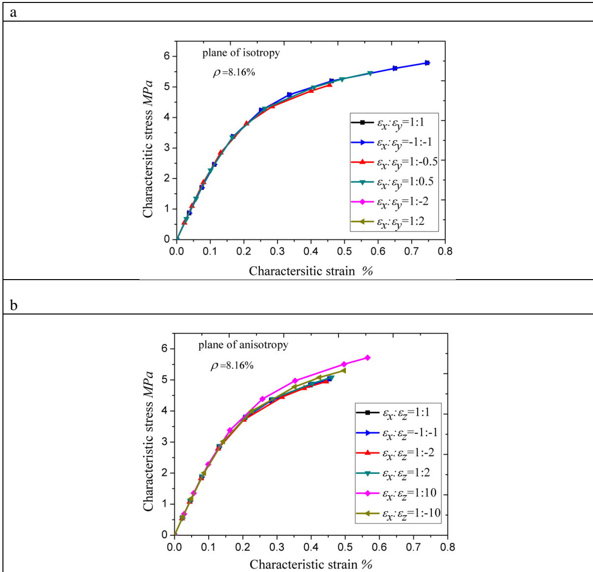
Fig.9. Characteristic stress-strain relations under biaxial loading in (a) plane of isotropy and (b) plane of anisotropy.
