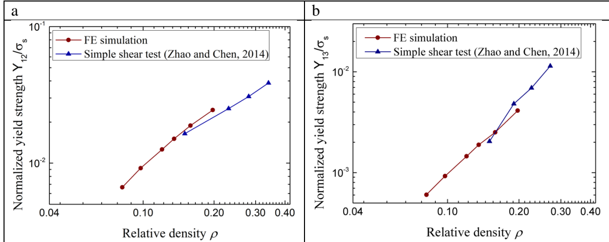
Fig.12. The effects of relative density on the shear strength of stochastic fibre network
