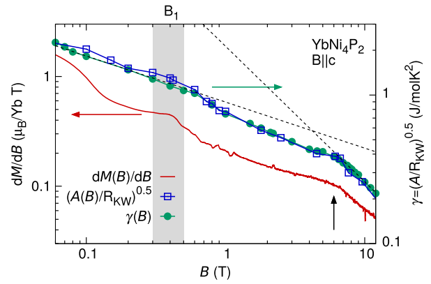
FIG. 3. Field dependence of the effective mass above B_c . As a measure of the effective mass, we plot here the field derivative of the magnetization dM/dB , the specific heat coefficient \gamma(B) , and the square root of the A coefficient of the resistivity in a double-logarithmic plot. The dashed lines highlight the change of slope in \gamma(B) just above B_1 (gray bar) and around B_5 < B < B_7 (short arrow). The changes around the latter field scale are too broad in our measurements to be connected to a single B_i .
