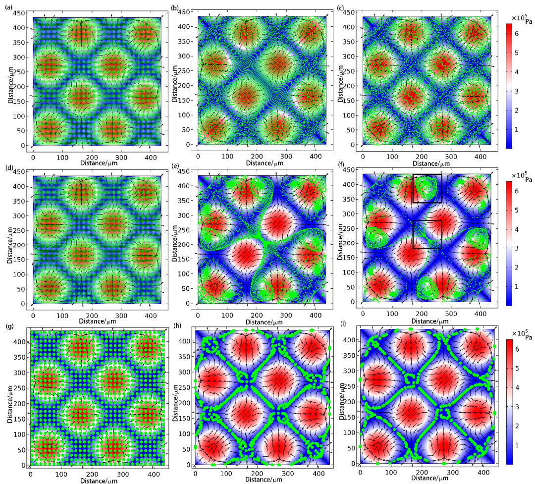
Figure 5. Simulation results in the continuous time with the arrows representing the flow velocity of the microfluidics, the color of the background the magnitude of the sound pressure in the standing wave field, and the green particles the polystyrene microspheres. (a–i) are the pattern of particles whose diameters are 1, 3, and 10 \mu\text{m} aggregation on different times. (To provide better visual effects, the 1 \mu\text{m} particles are zoomed in three times).
