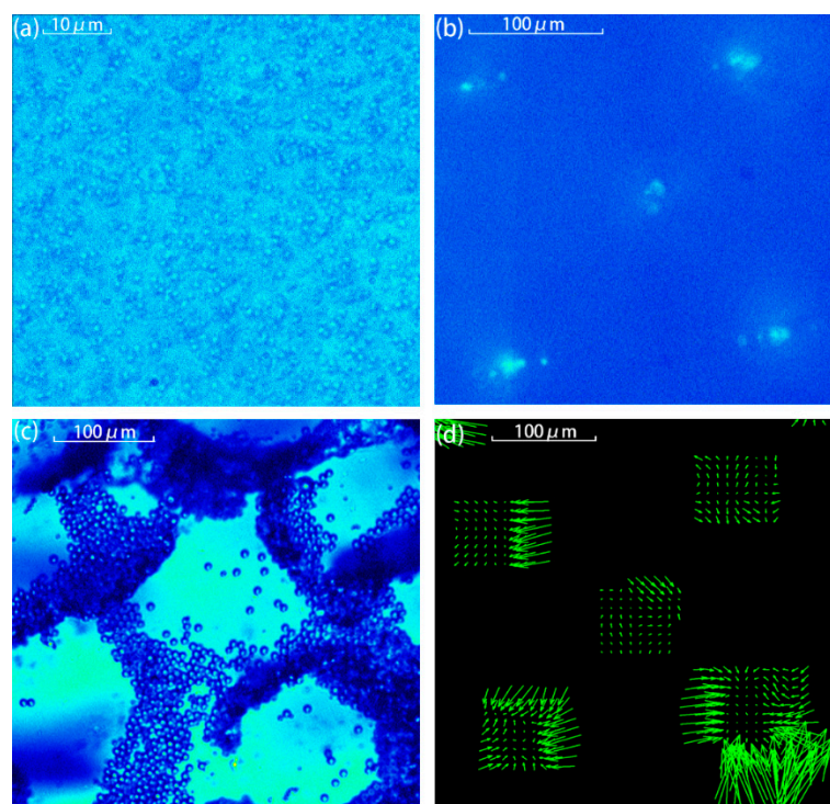
Figure 6. The two-dimension pattern of particles with a diameter of (a) 1 \mu\text{m} , (b) 3 \mu\text{m} , and (c) 10 \mu\text{m} . (d) is the velocity field from 3 \mu\text{m} particles measured by the PIV system.
