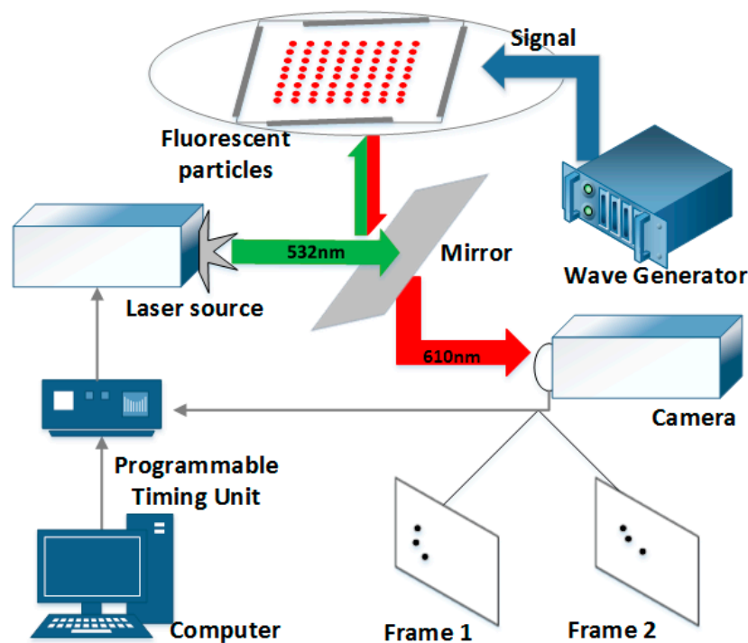
Figure 1. The experimental measurement system consisted of a signal electrical excitation system, a BAW microfluidic device, and a PIV system.
