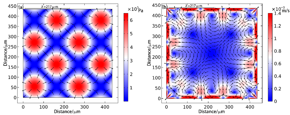
Figure 4. Simulation of two-dimensional particle patterning. In the figure (a), the background color represents the amplitude of the sound pressure, with blue for the node, red for the antinode, and the arrow indicating the direction of the sound radiation force. The figure (b) is the simulation result of microstreaming in the cavity, and the arrows represent the direction of the liquid flow and the background color represents the velocity of the microstreaming.
