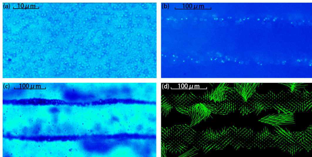
Figure 3. Experiment of one-dimension particle patterning (diameter = 1, 3, and 10 μm) is demonstrated in the (a–c) in sequence. The figure (d) is the 3 μm particle velocity field calculated by PIV system.
