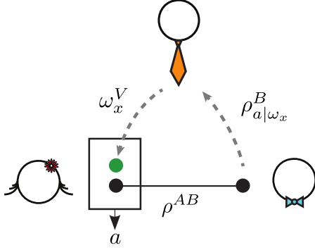
FIG. 1. Teleportation scenario: Alice and Bob share a bipartite state \rho^{AB} . A verifier, who wants to check whether this state is entangled, sends systems in one of the states \omega_x^V to Alice, and asks her to transmit it to Bob. Alice applies a global measurement on the state given to her by the verifier and her share of \rho^{AB} , which produces the states \rho_{a|\omega_x}^B for Bob. The verifier has to determine if \rho^{AB} is entangled based on the knowledge of \{\omega_x^V\}_x and \{\rho_{a|\omega_x}^B\}_{a,x} .
