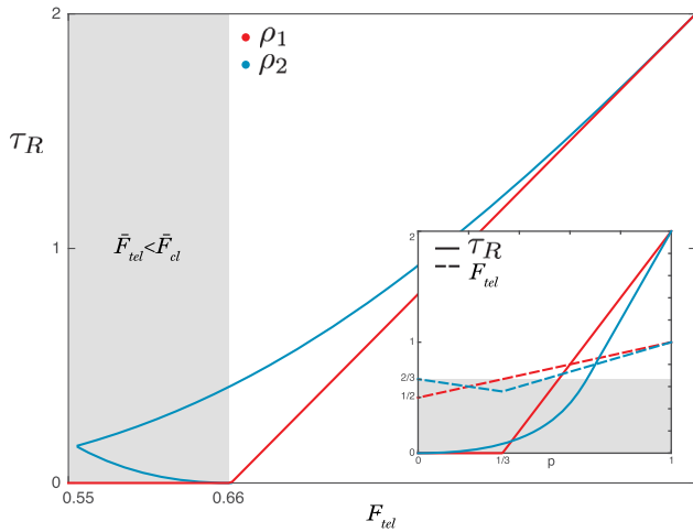
FIG. 2. Average fidelity of teleportation [33] versus random teleportation robustness for \rho_1^{AB} (red)—Eq. (11)—and \rho_2^{AB} (blue)—Eq. (12). The gray regions show the region where the average fidelity of teleportation is below the classical average fidelity \bar{F}_{cl} = 2/3 [34]. The inset shows the same quantities as a function of the noise parameter p for the two states.
