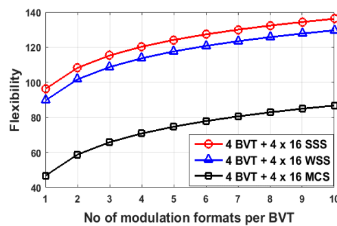
Fig. 16. Comparison of the flexibility of 4 x 16 WSS/MSC/SSS.
