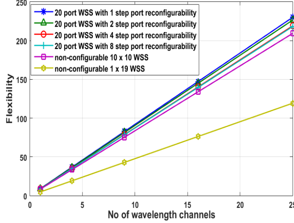
Fig. 7. Comparison of a non-configurable 1 \times 19 WSS, 10 \times 10 WSS and 20 port WSS of different steps of port reconfigurability.
