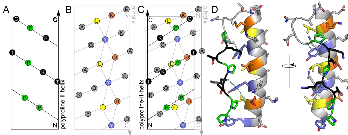
Figure 3: Design of PP \alpha combining polyproline II and \alpha -helices. A&B: 2D helical net representations (i.e. C \alpha atoms mapped onto cylinder of appropriate radii) of a canonical polyproline II helix ( A ) and \alpha -helix ( B ) and C: these two nets overlaid showing 'knobs-into-holes' packing of Pro and Tyr side chains. D: Representative NMR structure of PP \alpha -Tyr showing the CH- \pi interactions found (PDB: 5LO2). 19 Figure adapted from reference 19.
