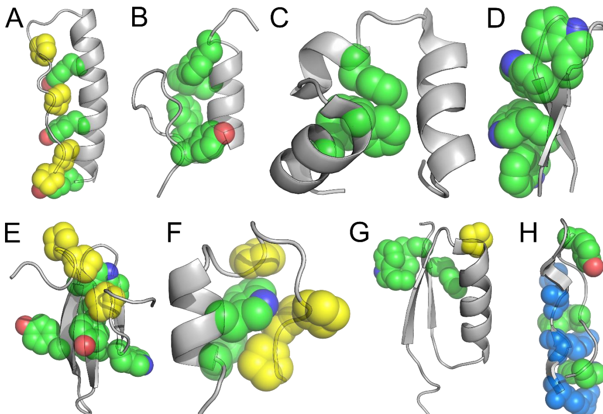
Figure 2: Miniprotein structures. A: PP \alpha -Tyr (PDB: 5LO2). 19 B: \beta\beta\alpha metal-free zinc finger (PDB: 1PSV). 26 C: Villin headpiece (PDB: 1YRI). 28 D: Trp-zipper \beta -hairpin (PDB: 1LE3). 29 E: Prototype WW domain (PDB: 1E0M). 30 F: Trp-cage (PDB: 2J0F). 31 G: \beta\alpha\beta (PDB: 2K10). H: TrpPlexus. 22 Structures are oriented N→C terminus left to right. Key: aromatics Trp, Tyr and Phe, green; Pro, yellow and Arg, light blue.
