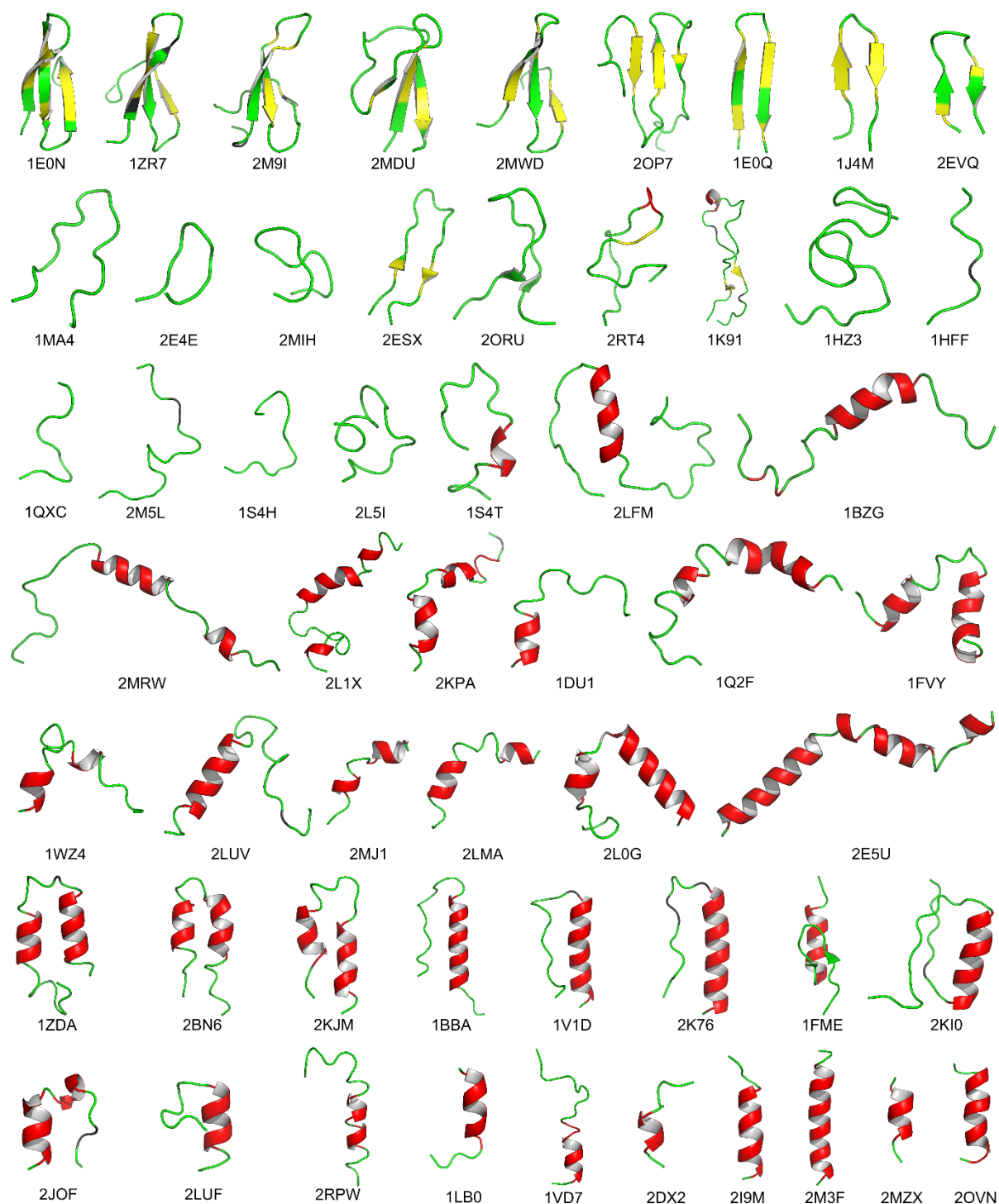
Figure 4: Non-redundant miniproteins. X-ray crystal and solution NMR structures of miniproteins downloaded from the PDB on 23/02/2017. Structures are arranged loosely by conformation, and oriented N \rightarrow C terminus left to right. For the solution-phase structures, this set includes only those determined in purely aqueous media. Key: \alpha helix, red; \beta strand, yellow; loop, green; and polyproline II helix, gray. N.B. DSSP assigns some regions of \beta hairpins and three-stranded \beta sheets as unstructured (green).
