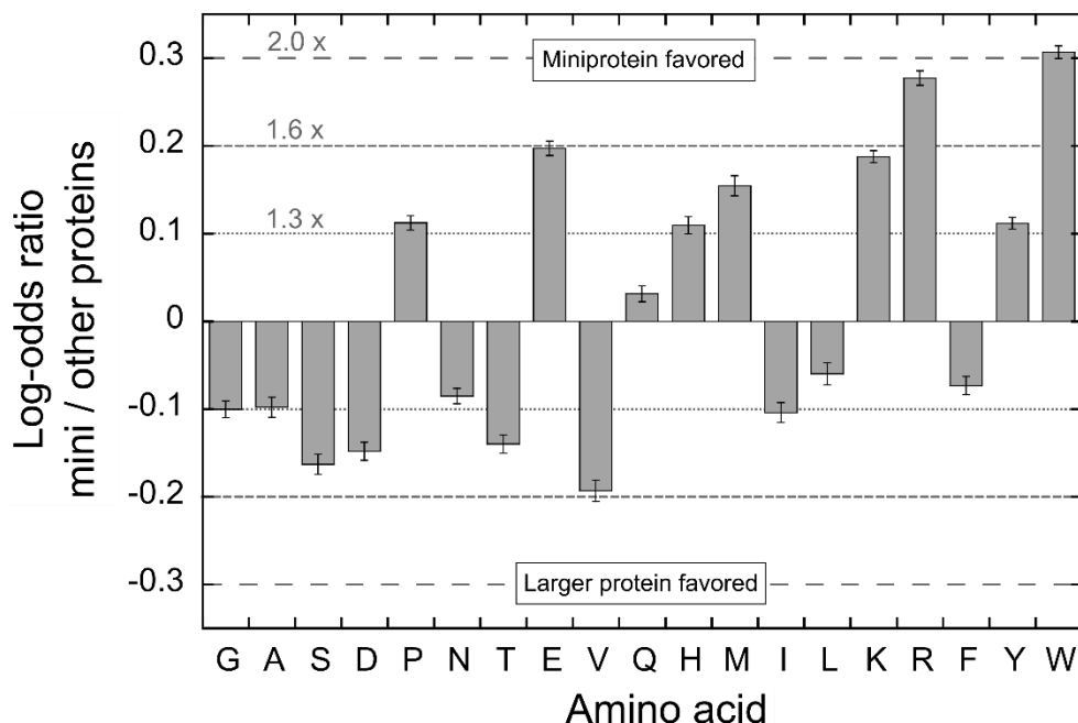
Figure 5: Amino-acid usage in miniproteins vs. larger proteins. These were calculated as the \log_{10} ratio of the normalized propensity of amino acids in miniproteins ( n = 55 ) vs. proteins \geq 100 residues long ( n = 120 ). Ratios of \pm 0.3 indicate a two-fold preference (long dashed lines); \pm 0.2 a 1.6-fold preference (short dashed lines); and \pm 0.1 a 1.3-fold preference (dotted lines). Amino acids are ordered by increasing side chain volume.
