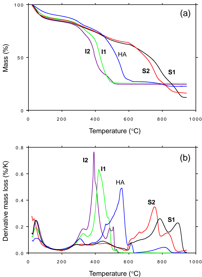
3 4 Fig. 2. (a) TG and (b) DTG profiles obtained in air for HA and the solubility fractions S1 , S2 , I1 and I2 .
