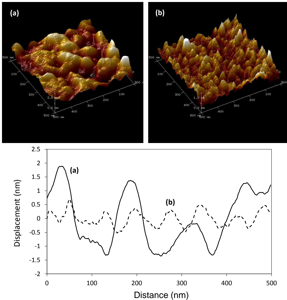
2 Fig. 6. Tapping mode 3-D topological AFM images (top) and section profiles through the respective AFM 3 images (bottom) for mica containing adsorbed SI from (a) ~0.5 g/L and (b) ~6 g/L solutions in deionized water 4 (see also Fig. 1(a) for the solutions used).
