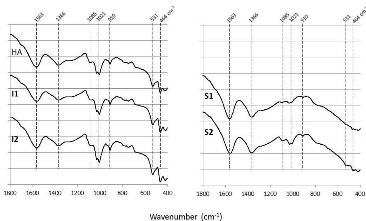
10 11 Fig. 3. ATR-IR spectra of original HA and its soluble and insoluble fractions (indicated). Arbitrary, but 12 constant, vertical transmittance scale.
