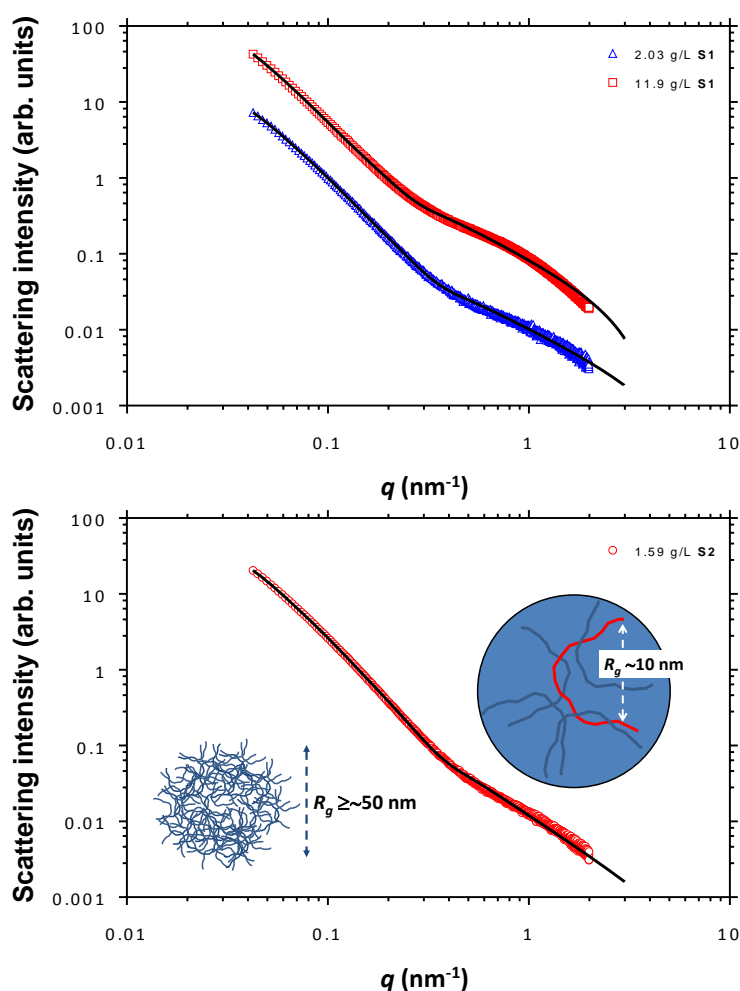
8 9 Fig. 7. SAXS Porod plots for S1 (upper) and S2 (lower) solutions at the indicated concentrations in deionized 10 water. The solid lines are unified (power law and Guinier) fits to the data (see text for details). The lower plot 11 also contains schematic representations of the length scales probed by the SAXS measurements.
