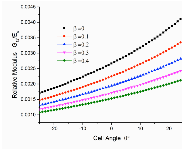
Figure 11 – Effect of the wall base ‘a’ ( \beta = a/l ). Non-dimensional shear modulus ( G_{12}/E_s ) vs internal cell angle for different wall base aspect ratios ( \beta = a/l ) for a=1 , \gamma=0.2 and \varphi=20^\circ .
