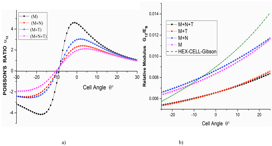
Figure 7 – Poisson's ratio and relative modulus of elasticity vs cell internal angle. (a): Influence of the cell internal angle on Poisson's ratio for \alpha=1, \beta=0.2 and \varphi=45^\circ .
