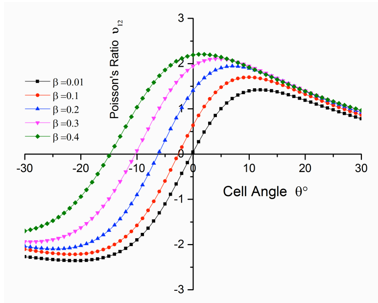
Figure 9 – Poisson's ratio ( \nu_{12} ) vs internal cell angle ( \theta ) and wall base aspect ratio ( \beta=a/l ).
