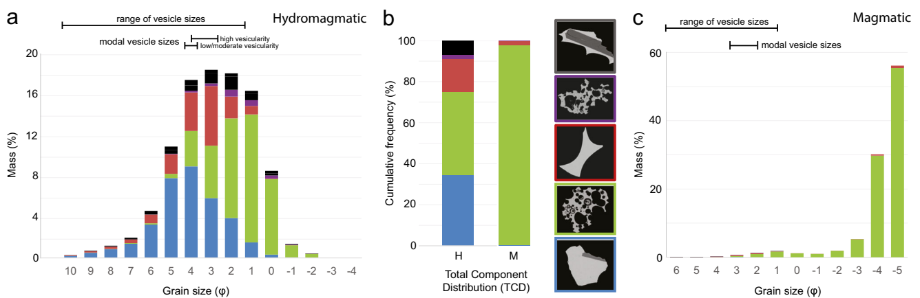
Fig. 12 a Total grain size distributions (TGSD) for the hydromagmatic fall and c GSD for a proximal magmatic scoria deposit [site Q1], showing the contributions of dense fragments (blue), vesicular particles (green), shards (red), microcrystalline grains (purple) and free crystals/lithics (black) to each size fraction (averaged over samples from a range of dispersal distances). Colour scheme is identical to Fig. 8. The range and
