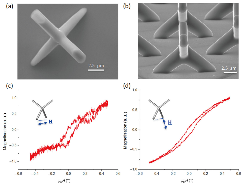
Figure S1 Tetrapod structures of larger feature size. (a) Scanning electron microscopy image of larger tetrapod structures (top view). (b) Scanning electron microscopy image of a larger tetrapod taken after 45° out-of-plane substrate rotation. Longitudinal MOKE loop of large tetrapod array with (c) field applied along projection of lower wires and (d) tetrapod array with field applied along projection of upper wires.
