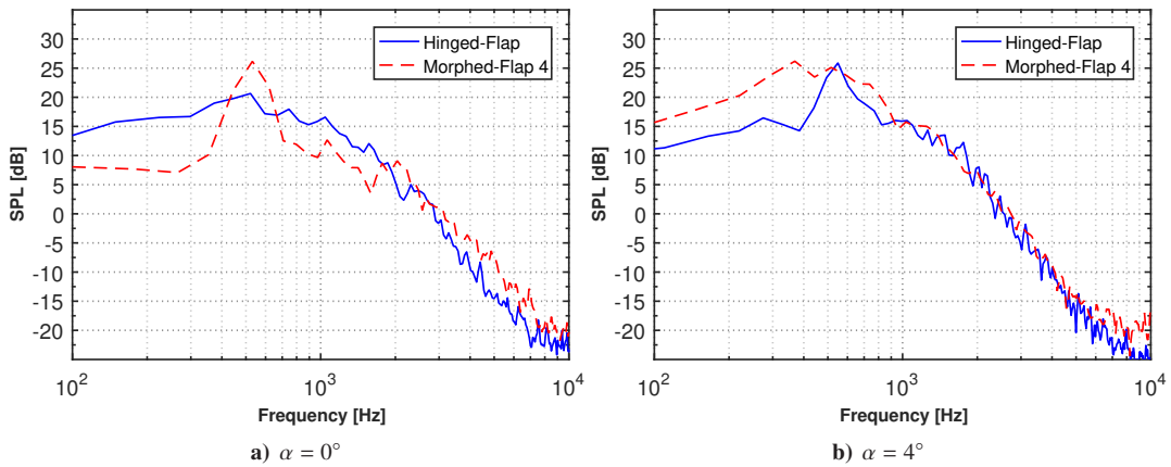
Fig. 17. Acoustic prediction using Curle's analogy, sound pressure level in dB reference to 2 \times 10^5 Pa, at the location 1.2 m above the trailing-edge for Hinged Flap and Morphed Flap 4 airfoils at angles of attack \alpha = 0^\circ and 4^\circ .
