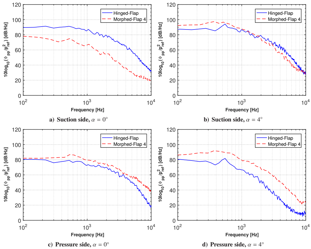
Fig. 16. Suction and pressure side wall-pressure spectra with reference to 2 \times 10^5 Pa, at the location x = 0.95c for Hinged Flap and Morphed Flap 4 airfoils at angles of attack \alpha = 0^\circ and 4^\circ .
