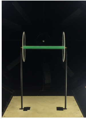
Fig. 2. NACA 0012 airfoil with side-plates set up in the wind tunnel.
