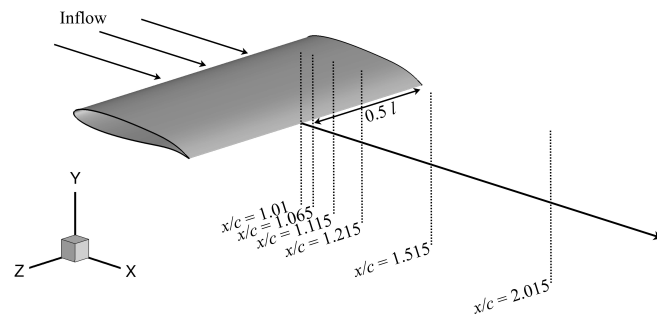
Fig. 7. Airfoil coordinate system along with wake velocity measurements locations.
