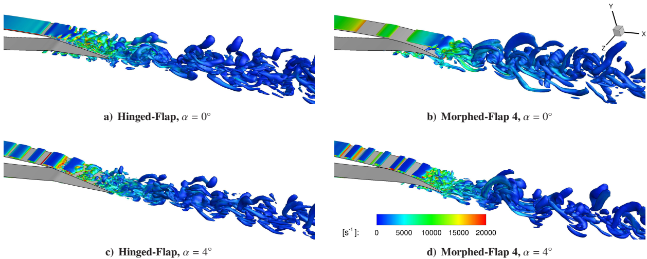
Fig. 11. Iso-surfaces of Q-criterion of Q = 1 \times 10^5 s^{-2} for Hinged Flap and Morphed Flap 4 airfoil with contours of vorticity magnitude.
